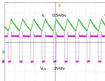
Time (1us/div)
