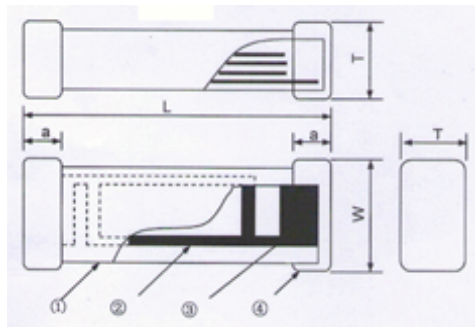
Ferrite for Series of inductors Internal electrode(Ag) Pull out electrode(Ag)
