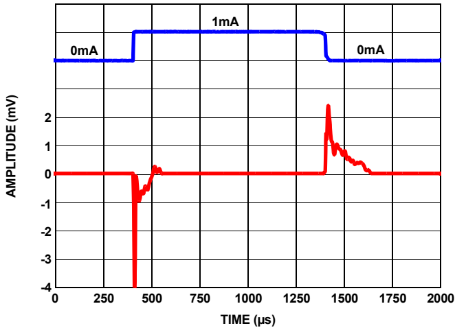
FIGURE 10. LOAD TRANSIENT RESPONSE AT 1mA LOAD AT 1µF
