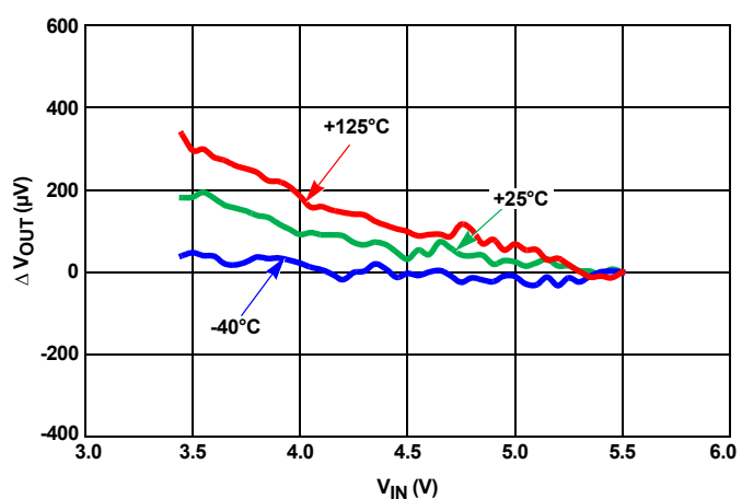
FIGURE 107. LINE REGULATION OVER-TEMPERATURE
