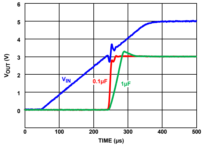
FIGURE 96. TURN-ON TIME
