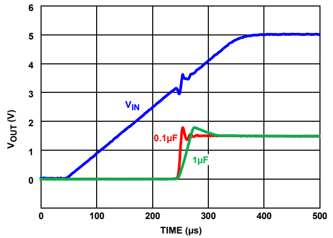
FIGURE 45. TURN-ON TIME
