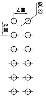
PCB LAYOUT
