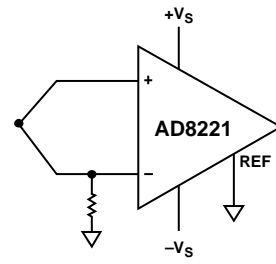
THERMOCOUPLE
