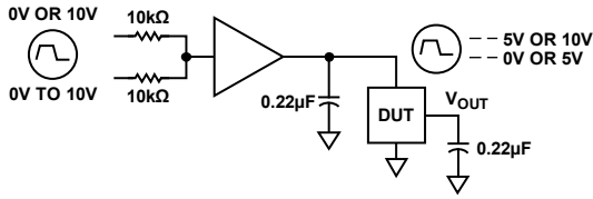
Figure 22. Turn-On/Transient Response Test Circuit
