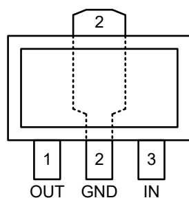
CJ6330AxxPT SOT-89-3L
