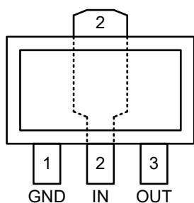
CJ6330AxxP SOT-89-3L
