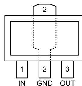
CJ6330AxxPL SOT-89-3L
