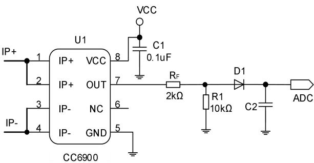
Rectifier output, instead of current transformer application
