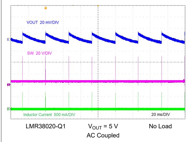
Figure 8-5. PFM Switching
