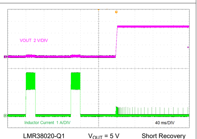
Figure 8-8. Short-Circuit Recovery
