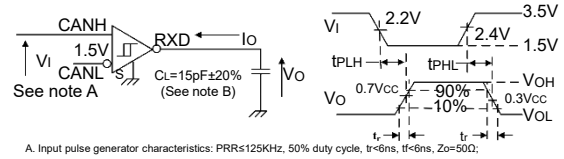
F6. Receiver test circuit and voltage waveform
