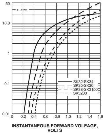
FIG. 3-TYPICAL INSTANTANEOUS FORWARD CHARACTERISTICS
