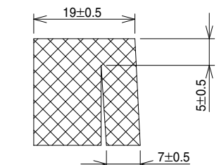
■Copper tape cut dimension
