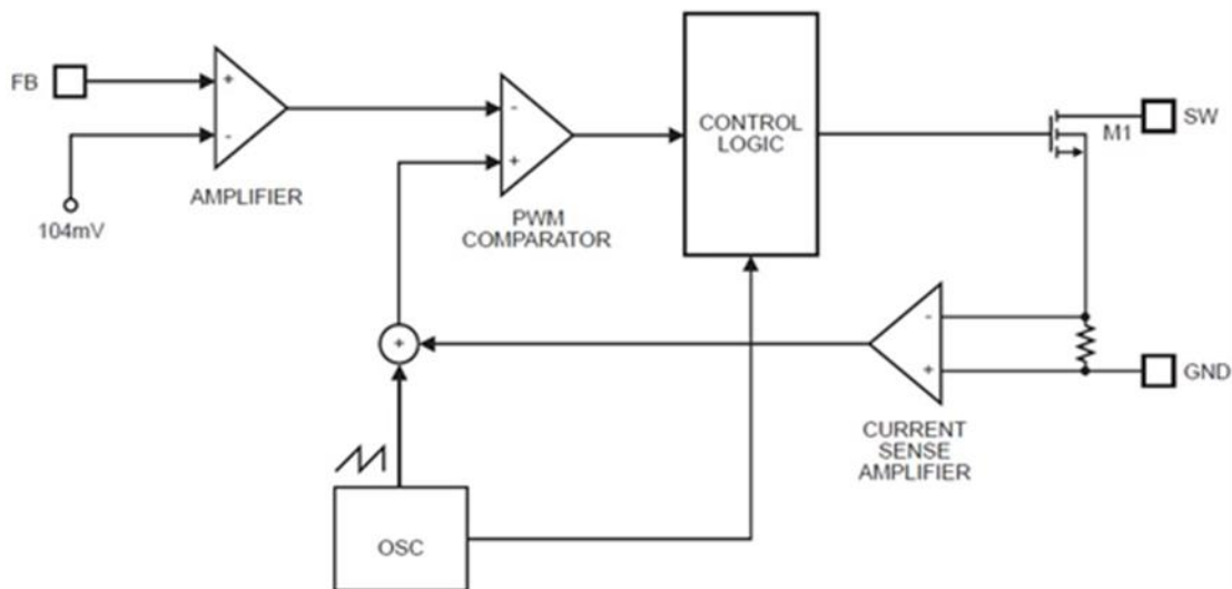
Figure 2. STI9287 Block Diagram
