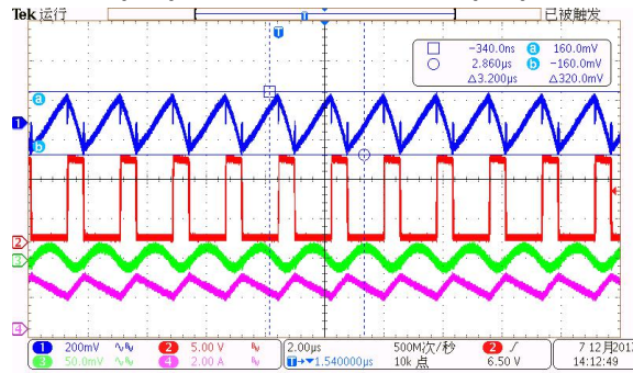
CH1:VIN(AC);CH2:SW;CH3:VOUT(AC);CH4:lsww
