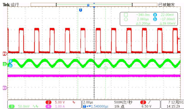
CH2:SW;CH3:VOUT(AC);CH4:lout
