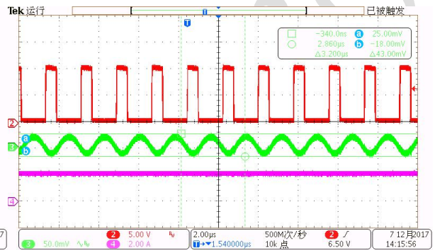
CH2:SW;CH3:VOUT(AC);CH4:lout
