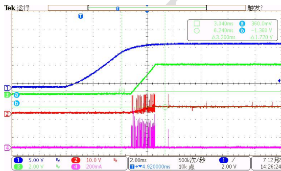
Power on, lout=0A
