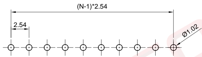
Recommend PCB Layout
