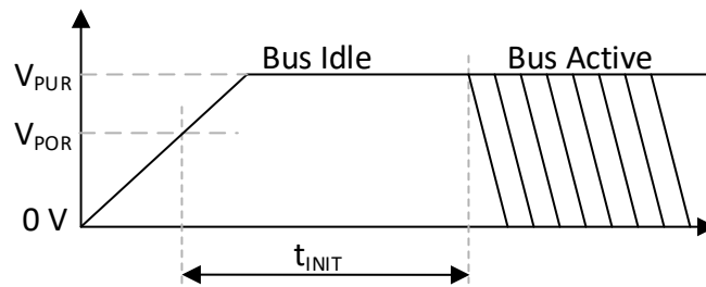
Figure 8-5. Bus Powered Initialization Timing Diagram
