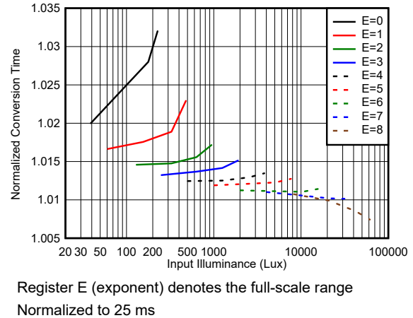
Figure 5-9. Conversion Time at 25 ms vs Input Light Level
