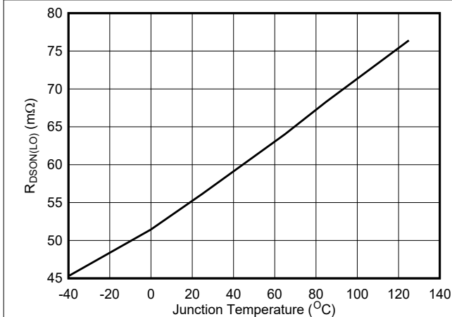
Figure 5-5. Low-Side Rdson
