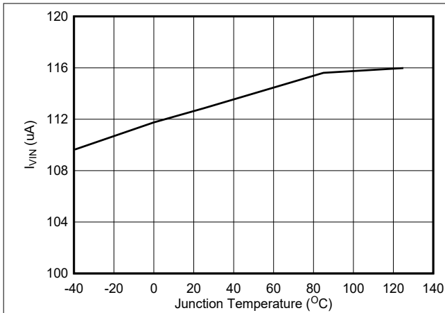
Figure 5-1. TPS563203 Quiescent Current
