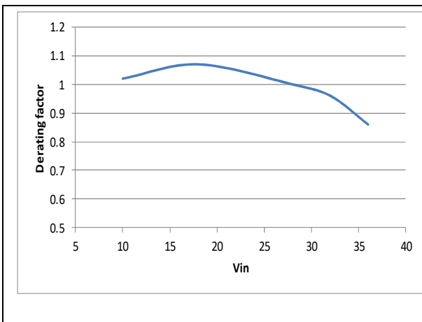
GQA2W024A050V typical temperature derating versus input voltage output with 2m/s (400 lfm) airflow from pin 3 to pin 1.
