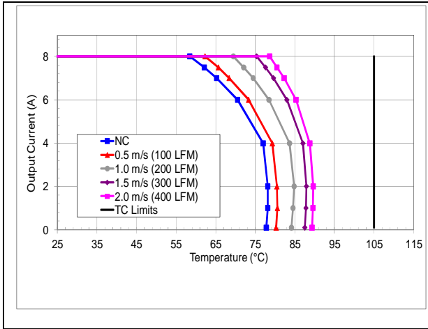
GQA2W008A150V maximum output current vs. ambient temperature at 28V input for airflow rates natural convection (60lfm) to 400lfm with airflow from pin 3 to pin 1
