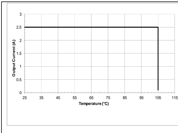
GQA24003A480V maximum output current vs. baseplate temperature
