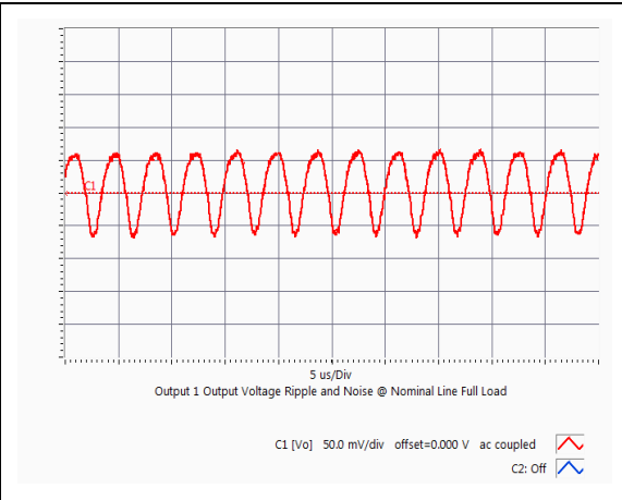
GQA24003A480V Typical Output Ripple at nominal Input voltage and full load at Ta=25 degree
