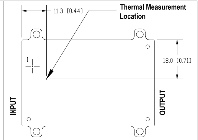
GQA2W004A280V-007 thermal measurement location – top view
