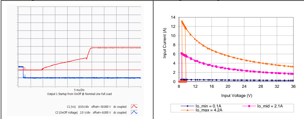
GQA2W004A280V Typical startup characteristic from on/off at full load. Blue trace - on/off signal, red trace - output voltage
