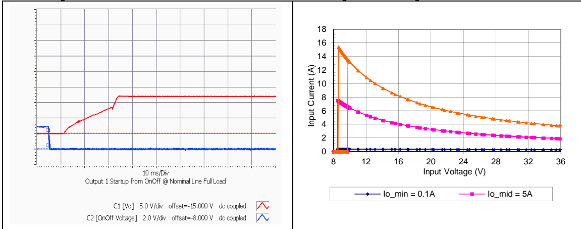
GQA2W010A120V Typical startup characteristic from on/off at full load. Lower trace - on/off signal, upper trace – output voltage
