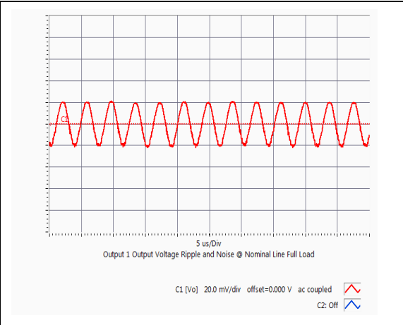
GQA2W024A050V Typical Output Ripple at nominal Input voltage and full load at Ta=25 degree
