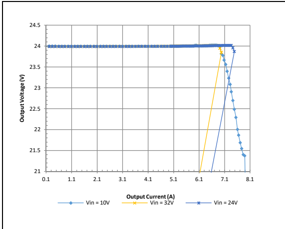
GQA2W005A240V Typical Output Current Limit Characteristics vs. Input Voltage at Ta=25 degrees.
