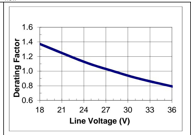
GQA24003A480V typical temperature derating versus input voltage output with 1m/s (200 lfm) airflow from pin 3 to pin 1.
