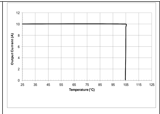
GQA2W010A120V maximum output current vs. baseplate temperature at nominal line
