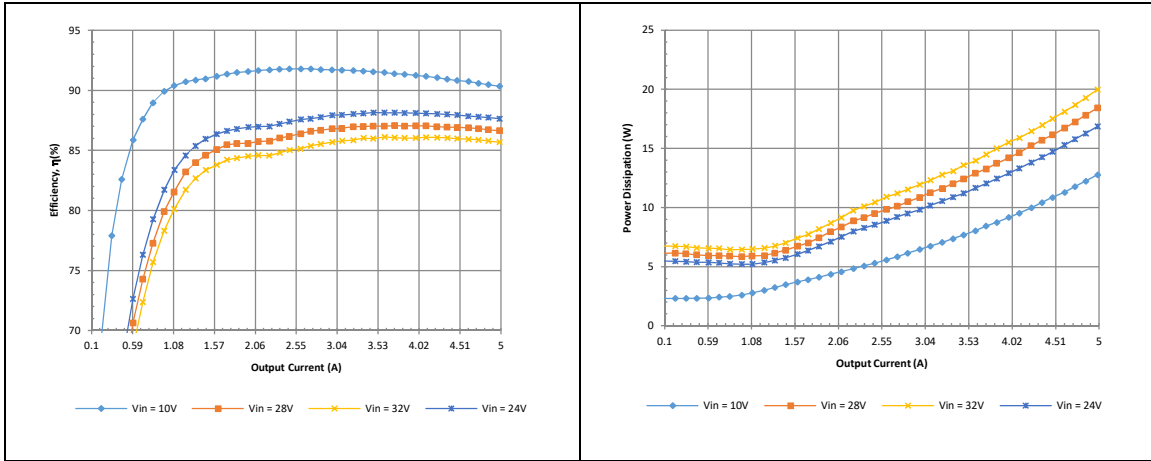
GQA2W005A240V Typical Efficiency vs. Input Voltage at Ta=25 degrees.
