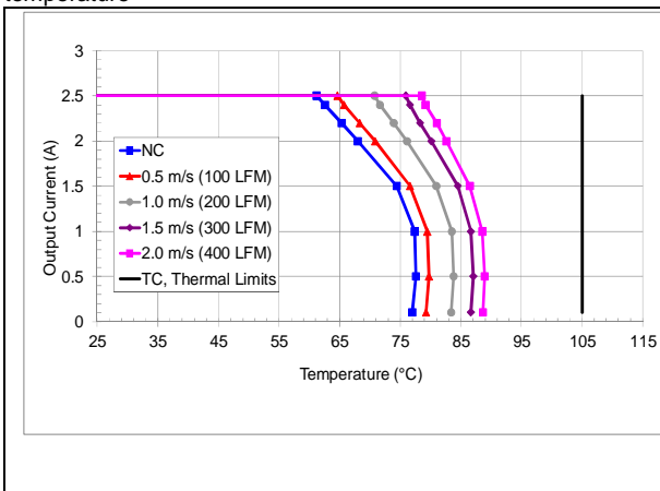
GQA24003A480V maximum output current vs. ambient temperature at 28V input for airflow rates natural convection (60lfm) to 400lfm with airflow from pin 3 to pin 1
