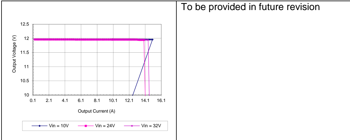
GQA2W010A120V Typical Output Current Limit Characteristics vs. Input Voltage at Ta=25 degrees.
