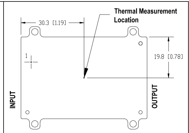
GQA2W024A050V thermal measurement location – top view
