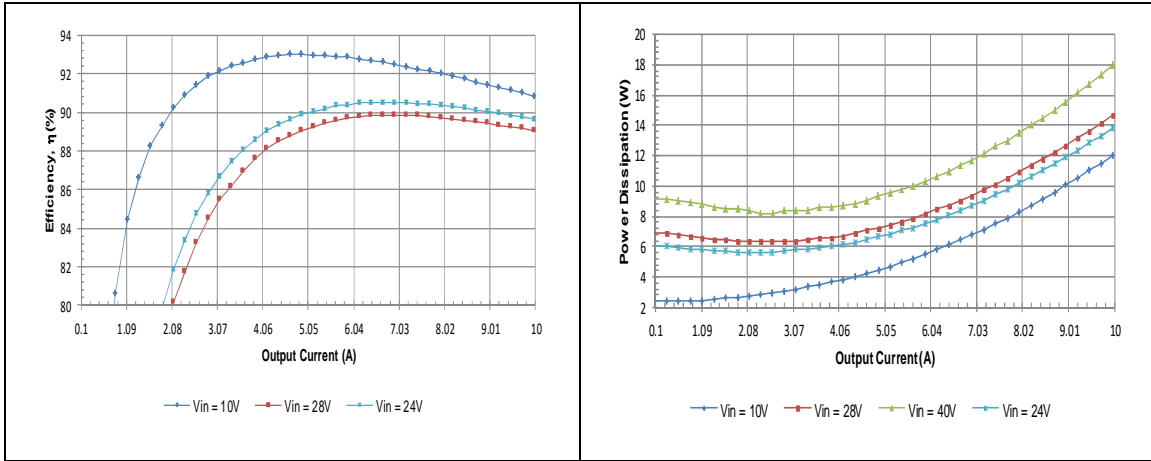
GQA2W010A120V Typical Efficiency vs. Input Voltage at T_a=25 degrees.
