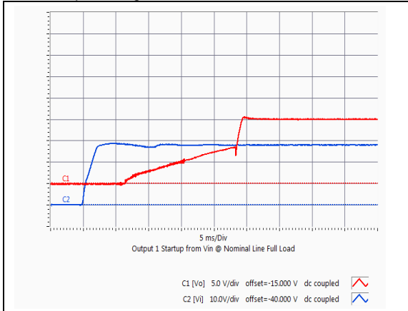
GQA2W008A150V Typical startup characteristic from input voltage application at full load. Red trace - output voltage, Blue trace - input voltage
