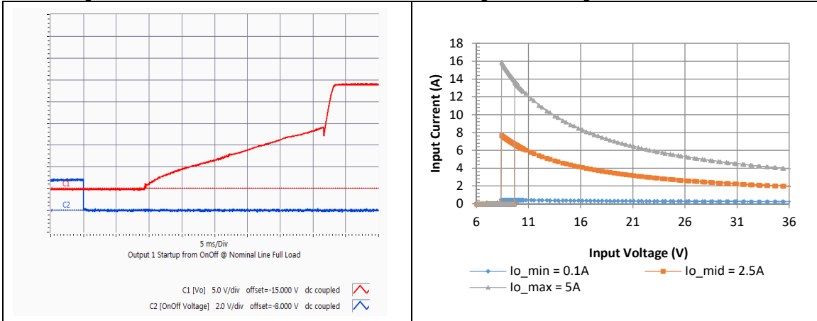
GQA2W005A240V Typical startup characteristic from on/off at full load. Blue trace - on/off signal, red trace - output voltage
