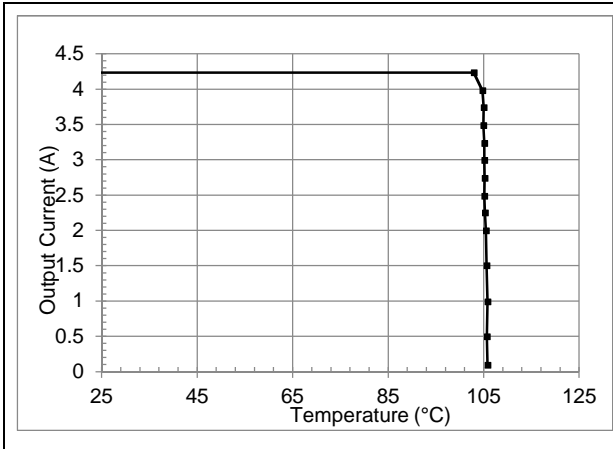
GQA2W004A280V maximum output current vs. baseplate temperature
