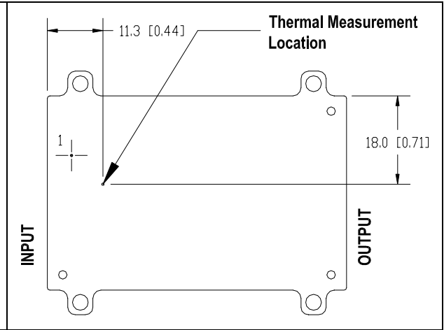
GQA2W008A150V thermal measurement location – top view
