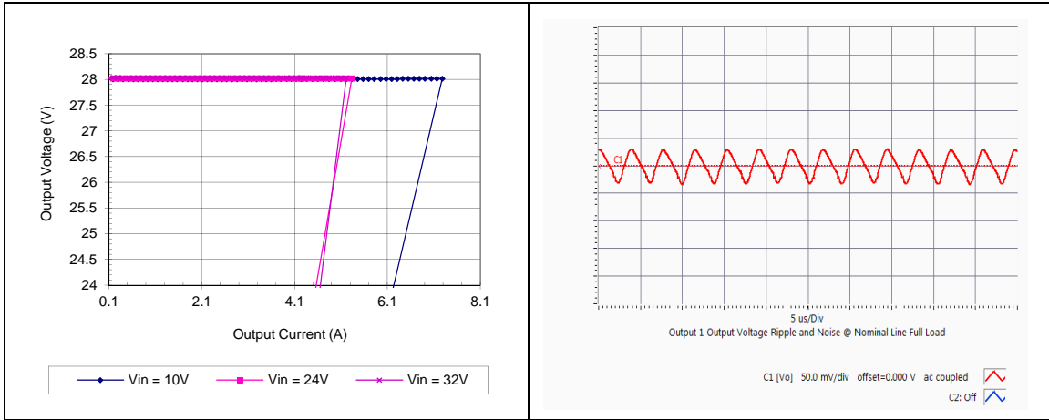
GQA2W004A280V Typical Output Current Limit Characteristics vs. Input Voltage at Ta=25 degrees.
