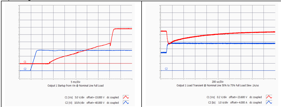
GQA2W005A240V Typical startup characteristic from input voltage application at full load. Red trace - output voltage, blue trace - input voltage
