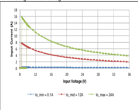
GQA2W024A050V Typical Input Current vs. Input Voltage Characteristics
