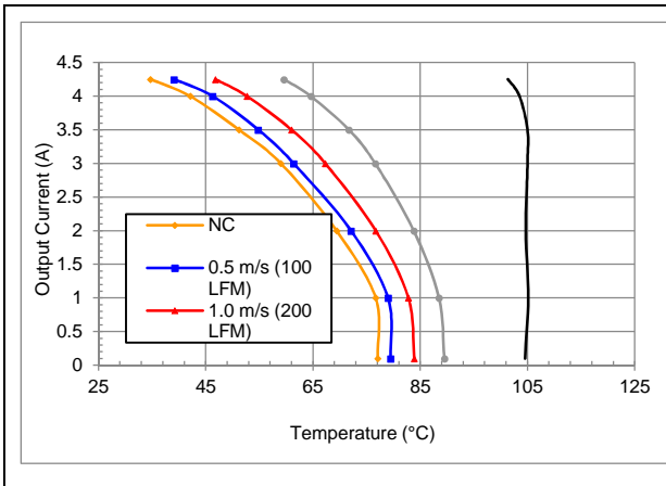
GQA2W004A280V maximum output current vs. ambient temperature at 28V input for airflow rates natural convection (60lfm) to 400lfm with airflow from pin 3 to pin 1.
