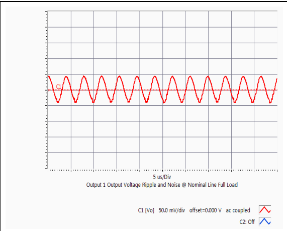
GQA2W005A240V Typical Output Ripple at nominal Input voltage and full load at Ta=25 degree
