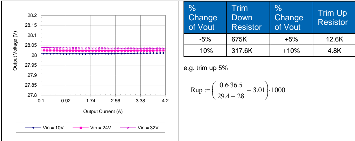
GQA2W004A280V Typical Load Regulation Characteristics at Ta=25 degrees.
