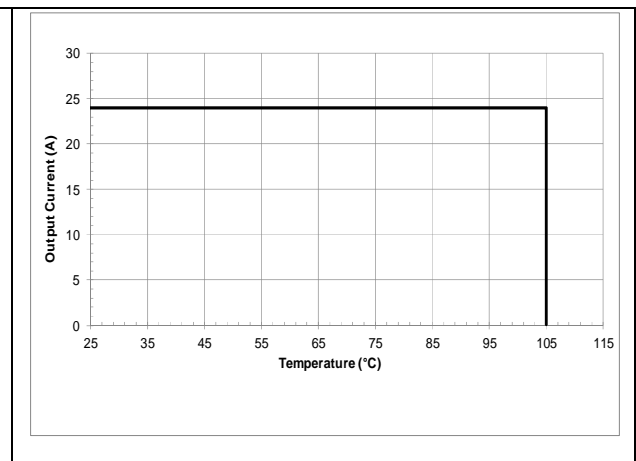
GQA2W024A050V maximum output current vs. baseplate temperature at nominal line
