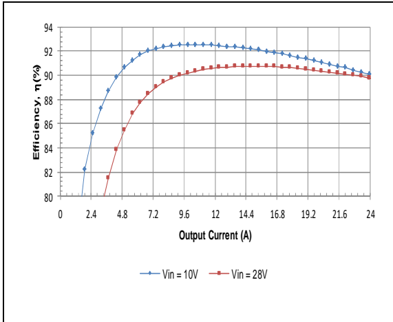
GQA2W024A050V Typical Efficiency vs. Input Voltage at Ta=25 degrees.
