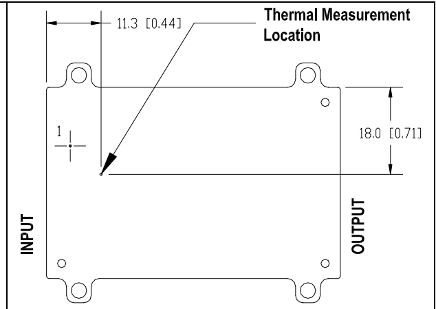
GQA2W010A120V thermal measurement location – top view
