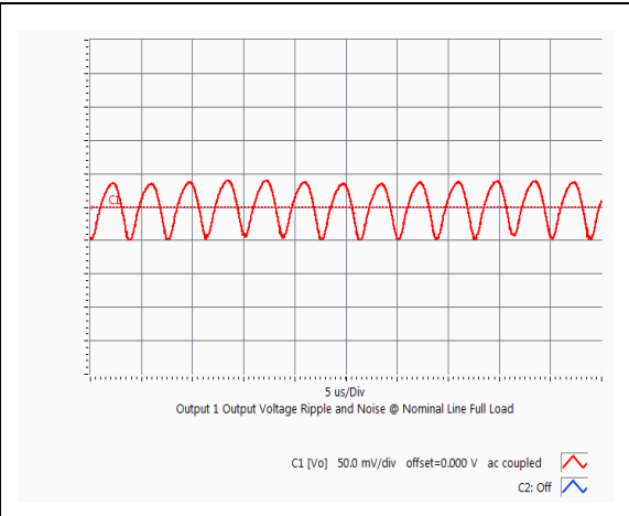
GQA2W008A150V Typical Output Ripple at nominal Input voltage and full load at Ta=25 degree
