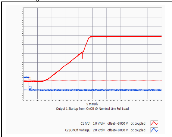
GQA2W024A050V Typical startup characteristic from on/off at full load. Lower trace - on/off signal, upper trace - output voltage
