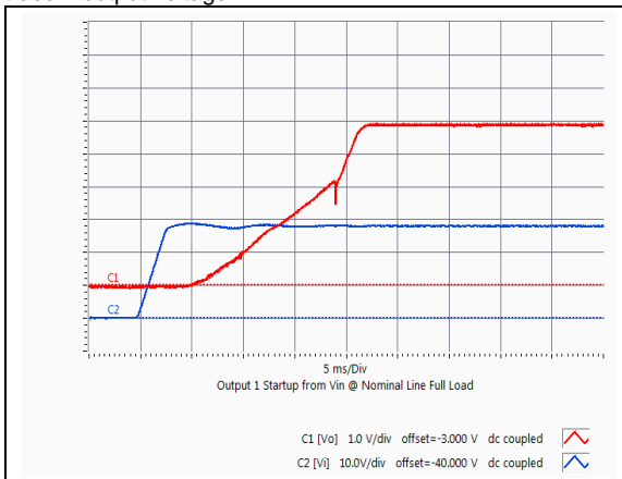
GQA2W024A050V Typical startup characteristic from input voltage application at full load. Red trace - output voltage, Blue trace - input voltage
