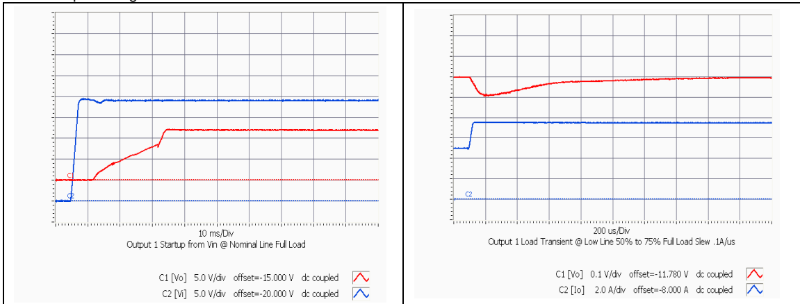
GQA2W010A120V Typical startup characteristic from input voltage application at full load. Red trace - output voltage, Blue trace - input voltage
