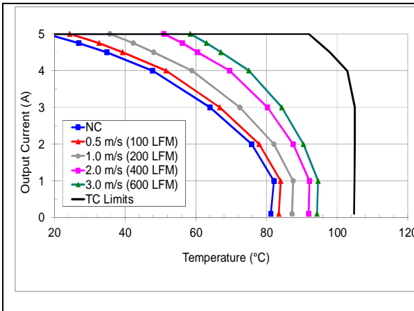
GQA2W005A240V maximum output current vs. ambient temperature at 28V input for airflow rates natural convection (60lfm) to 600lfm with airflow from pin 3 to pin 1.
