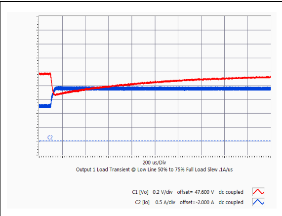
GQA24003A480V Typical transient response. Output voltage response to load step from 50% to 75% of full load with output current slew rate of 0.1A/us.
