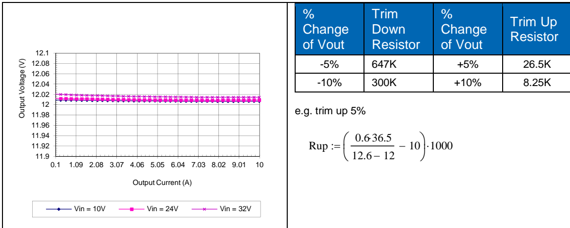
GQA2W010A120V Typical Load Regulation Characteristics at Ta=25 degrees.
