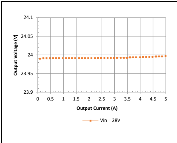
GQA2W005A240V Typical Load Regulation Characteristics at Ta=25 degrees.
