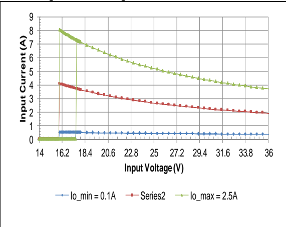
GQA24003A480V Typical Input Current vs. Input Voltage Characteristics
