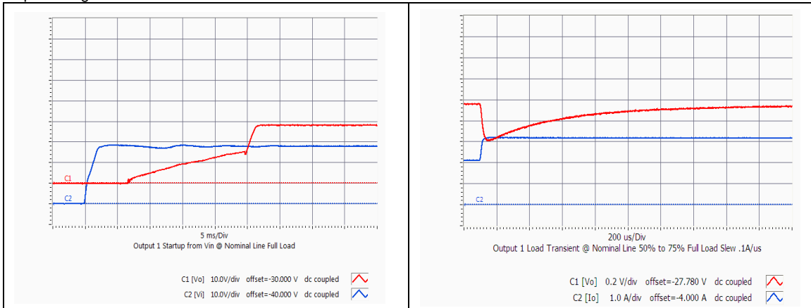
GQA2W004A280V Typical startup characteristic from input voltage application at full load. Red trace - output voltage, blue trace - input voltage
