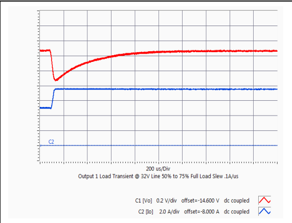
GQA2W008A150V Typical output voltage response to load step from 50% to 75% of full load with output current slew rate of 0.1A/uS and C_{ext} = 10\mu F
