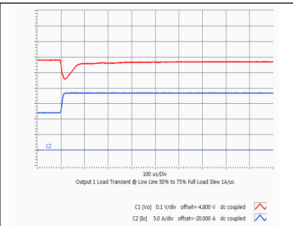
GQA2W024A050V Typical output voltage response to load step from 50% to 75% of full load with output current slew rate of 1A/uS and Cext = 22uF
