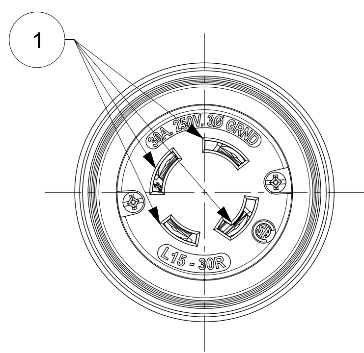
FACE VIEW
