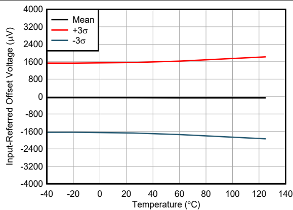
Figure 7-17. Offset Voltage (RTI) vs Temperature
