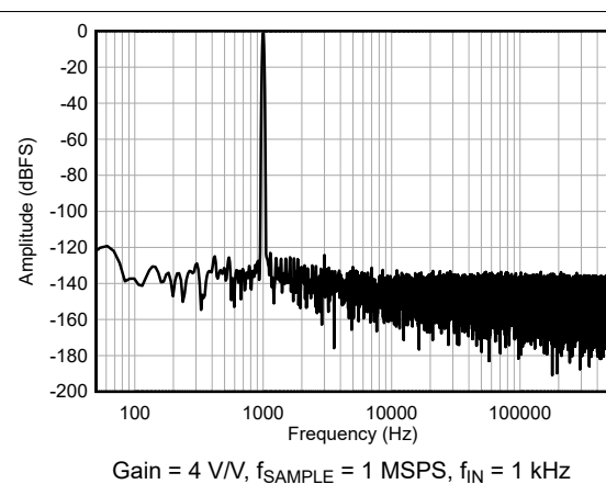
Figure 9-11. Performance FFT Plot With ADS8900B
