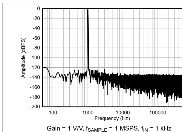
Figure 9-10. Performance FFT Plot With ADS8900B
