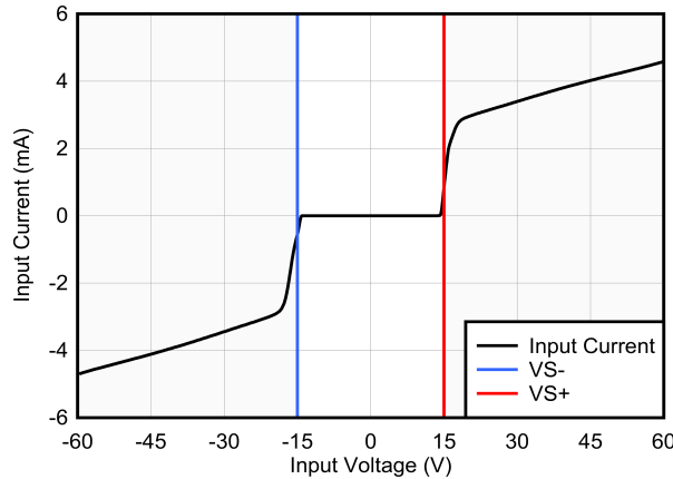
Figure 8-2. Input Current vs Input Overvoltage
