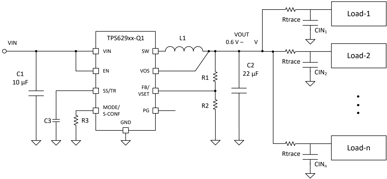
Figure 9-83. Multiple Loads
