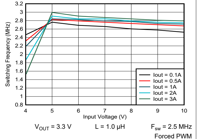
Figure 9-55. Switching Frequency vs Input Voltage
