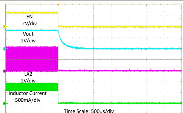
Figure 9-13. Shutdown by EN
