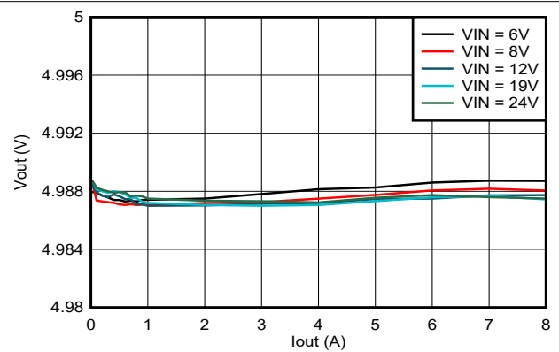
Figure 7-3. Load Regulation
