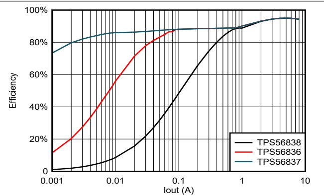
Figure 5-22. TPS56837, TPS56838 and TPS56836 Efficiency, V_{in} = 24V , V_{out} = 5V , F_{sw} = 500kHz
