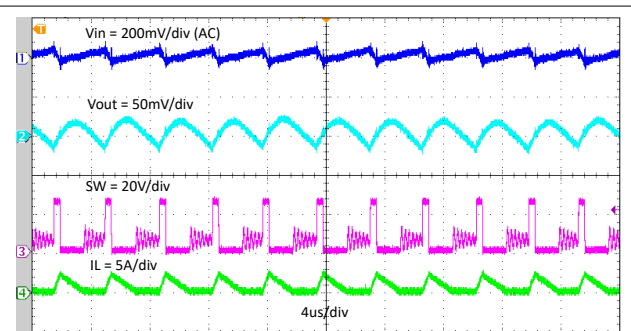
Figure 7-7. Steady State Waveforms, IOUT = 0.6A
