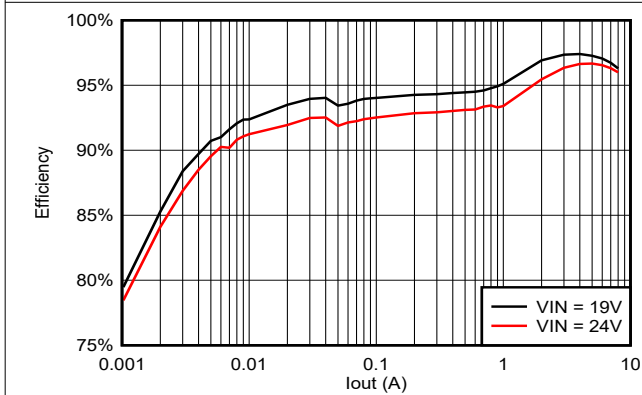
Figure 5-21. TPS56837 Efficiency, V_{out} = 12V , F_{sw} = 800kHz
