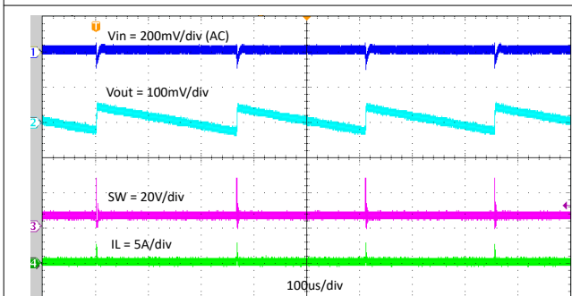
Figure 7-6. Steady State Waveforms, IOUT = 0.01A
