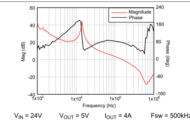
Figure 7-5. Bode Plot
