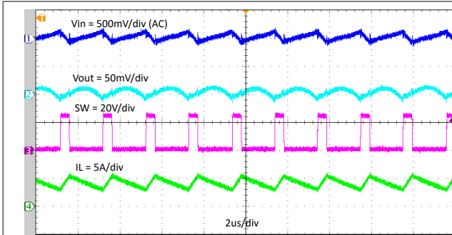
Figure 7-8. Steady State Waveforms, I_{OUT} = 4A
