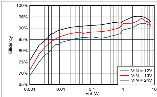
Figure 5-19. TPS56837 Efficiency, V_{out} = 5V , F_{sw} = 1200kHz
