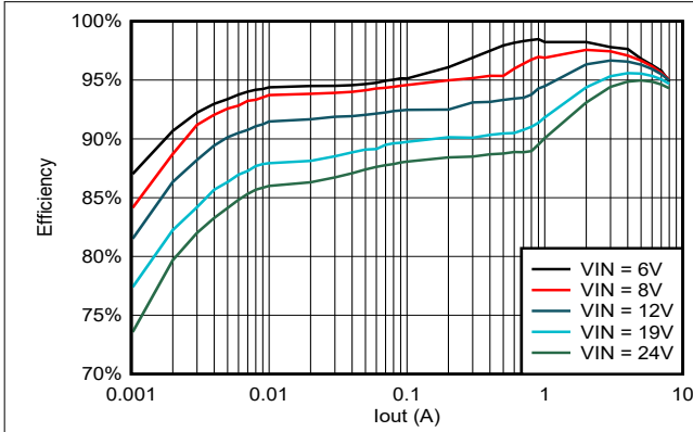
Figure 7-2. Efficiency
