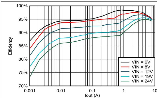
Figure 5-17. TPS56837 Efficiency, V_{out} = 5V , F_{sw} = 500kHz
