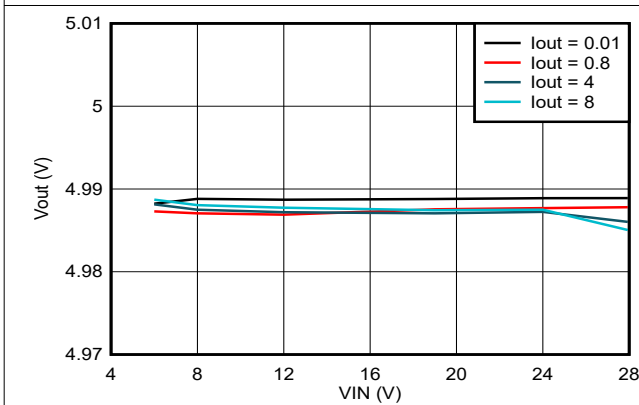
Figure 7-4. Line Regulation
