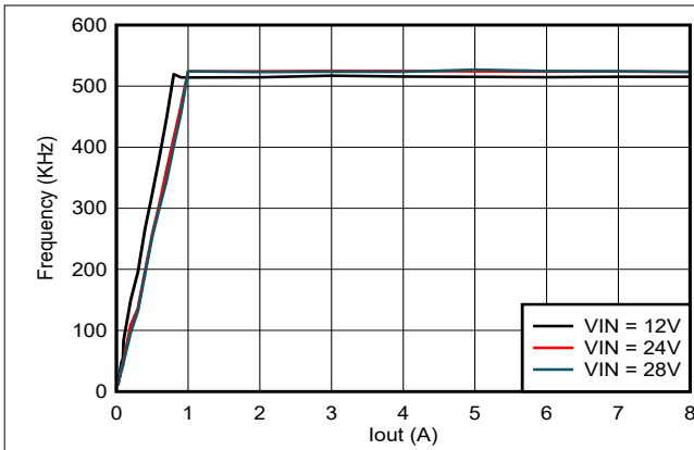
Figure 5-13. TPS56837 Switching Frequency vs Output Current, V_{out} = 5V , F_{sw} = 500kHz
