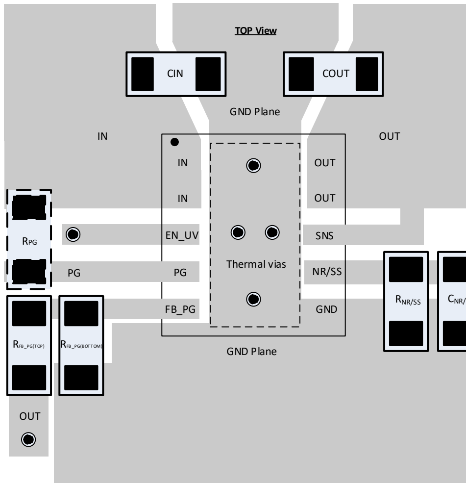
Figure 8-33. Example Layout
