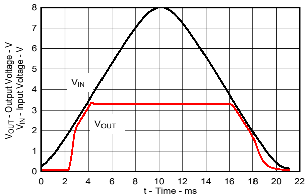
Figure 5-13. Power-Up, Power-Down With V_{IN} Ramp
