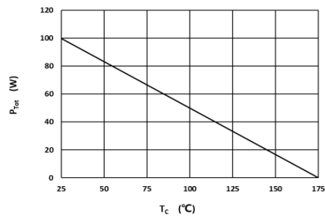
Fig 4: Power Derating
