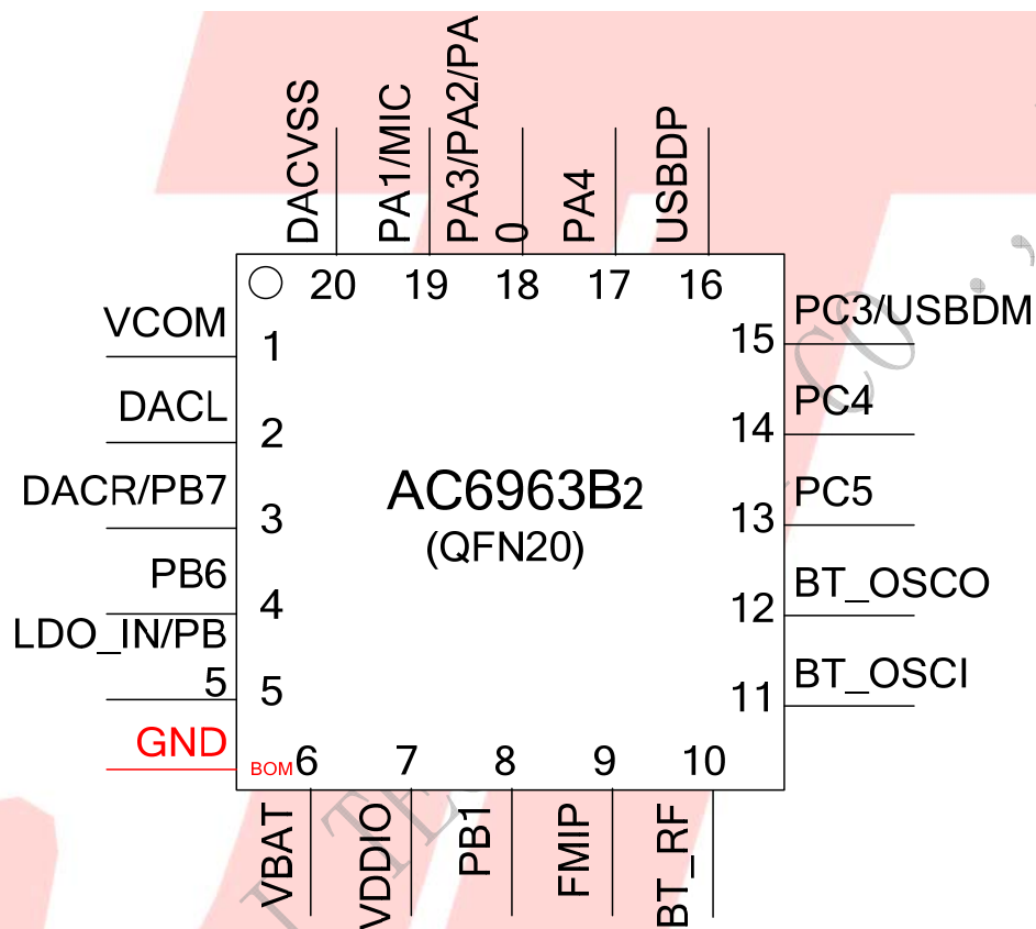
Figure 1-1 AC6963B_QFN20
