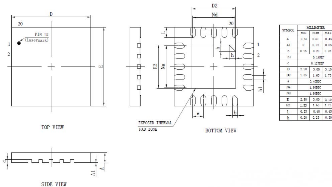
Figure 3-1. AC6963B_QFN20 Package
