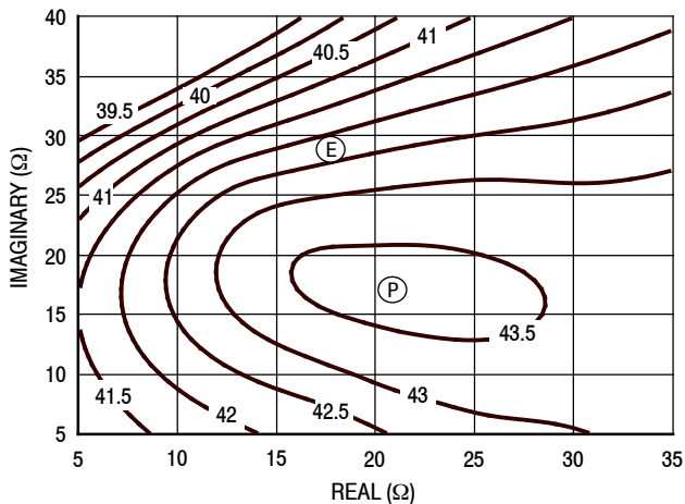
Figure 9. P1dB Load Pull Output Power Contours (dB)
