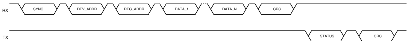
Figure 6-16. Multiple Data Bytes Write in Burst Mode
