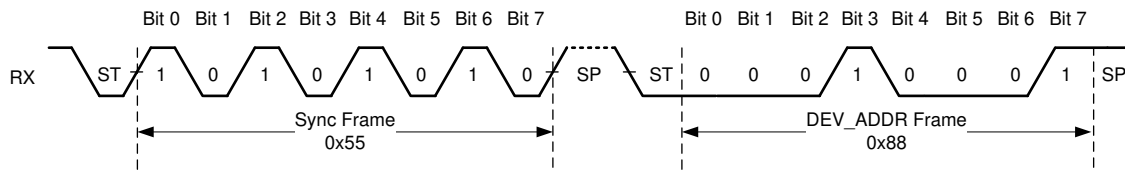
Figure 6-13. Synchronization Byte
