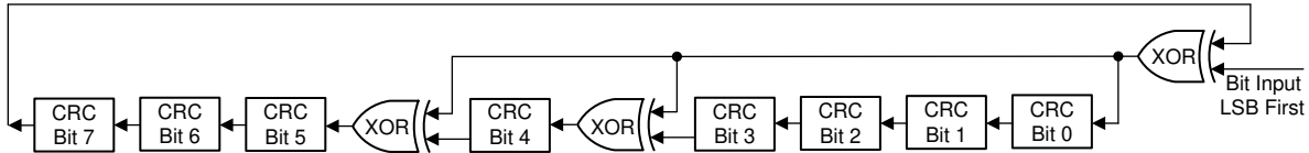
Figure 6-7. CRC Algorithm Diagram
