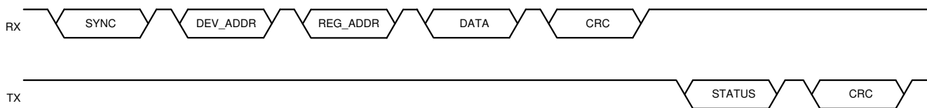
Figure 6-11. Single-Byte Write Command with Status Feedback
