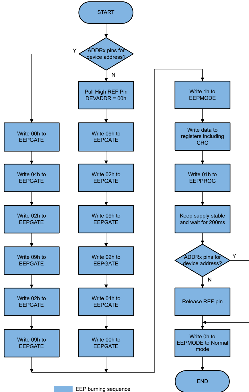
Figure 6-18. Programming Sequence
