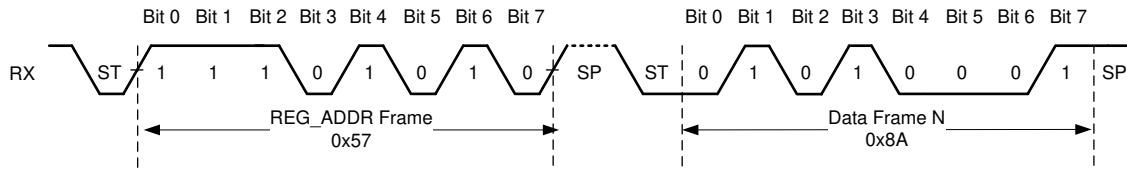
Figure 6-14. Address and Data Bytes
