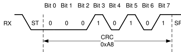
Figure 6-15. CRC Byte
