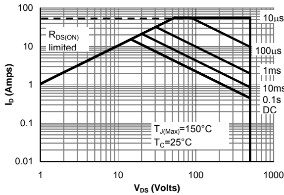
Figure 9: Maximum Forward Biased Safe Operating Area for AOT14N50 (Note F)
