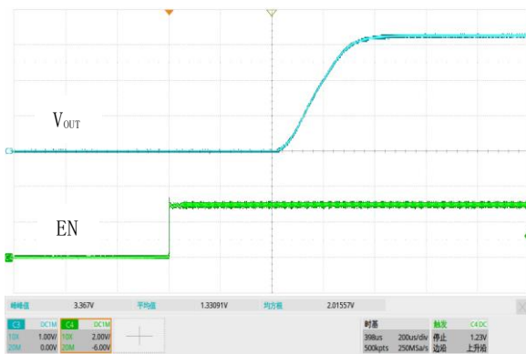
图 22. 软启动, V_{IN}=4.3V, V_{OUT}=3.3V, I_{OUT}=150mA
