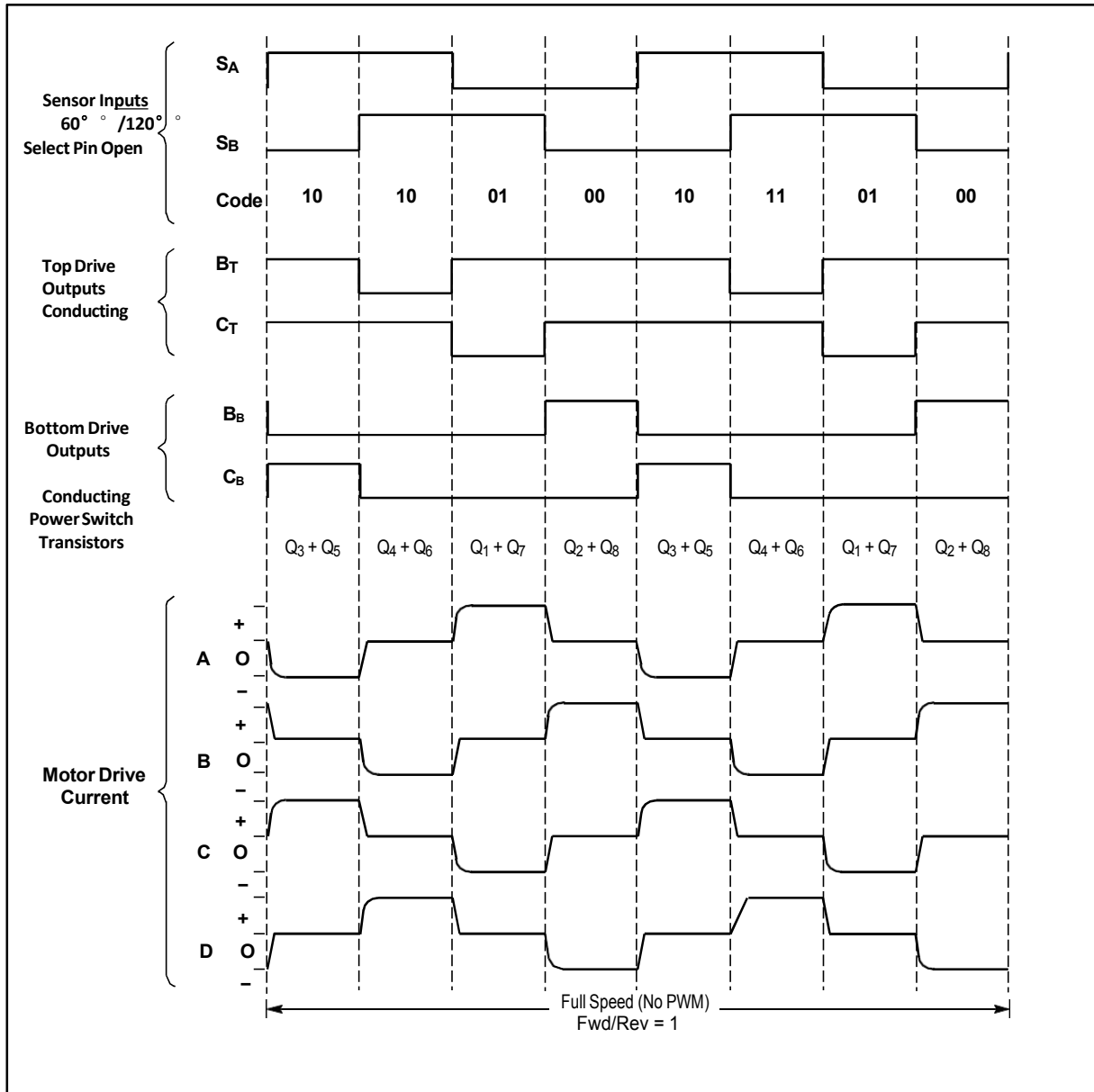
Figure 46. Four Phase, Four Step, Full Wave Motor Controller
