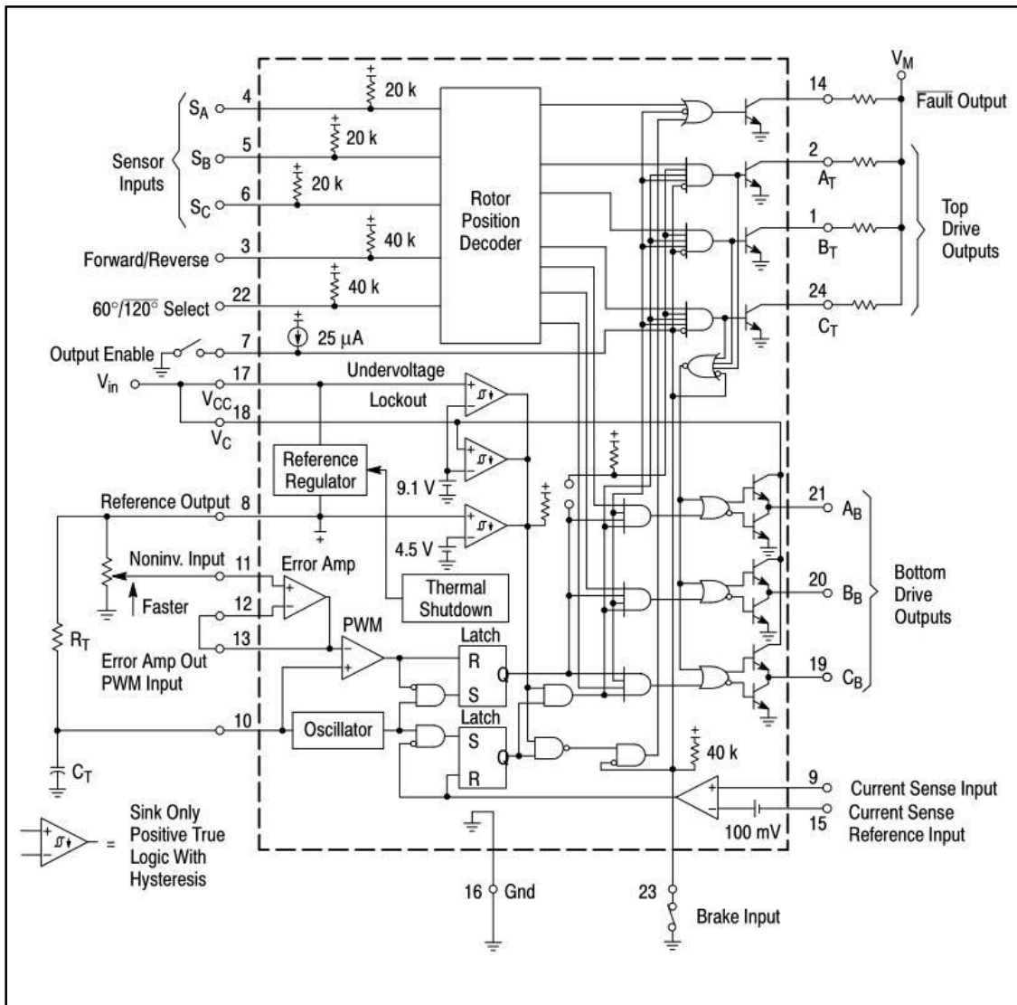
Figure 22. Representative Block Diagram
