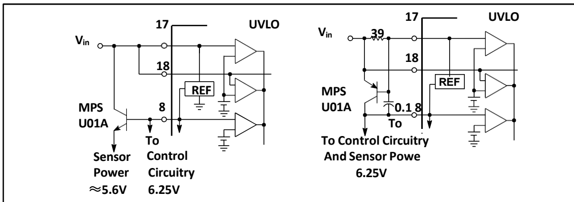
Figure 24. Reference Output Buffers
