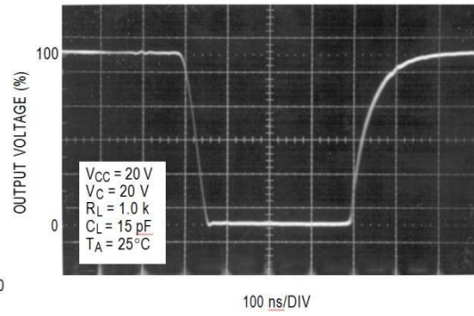
Figure 17. Top Drive Output Waveform
