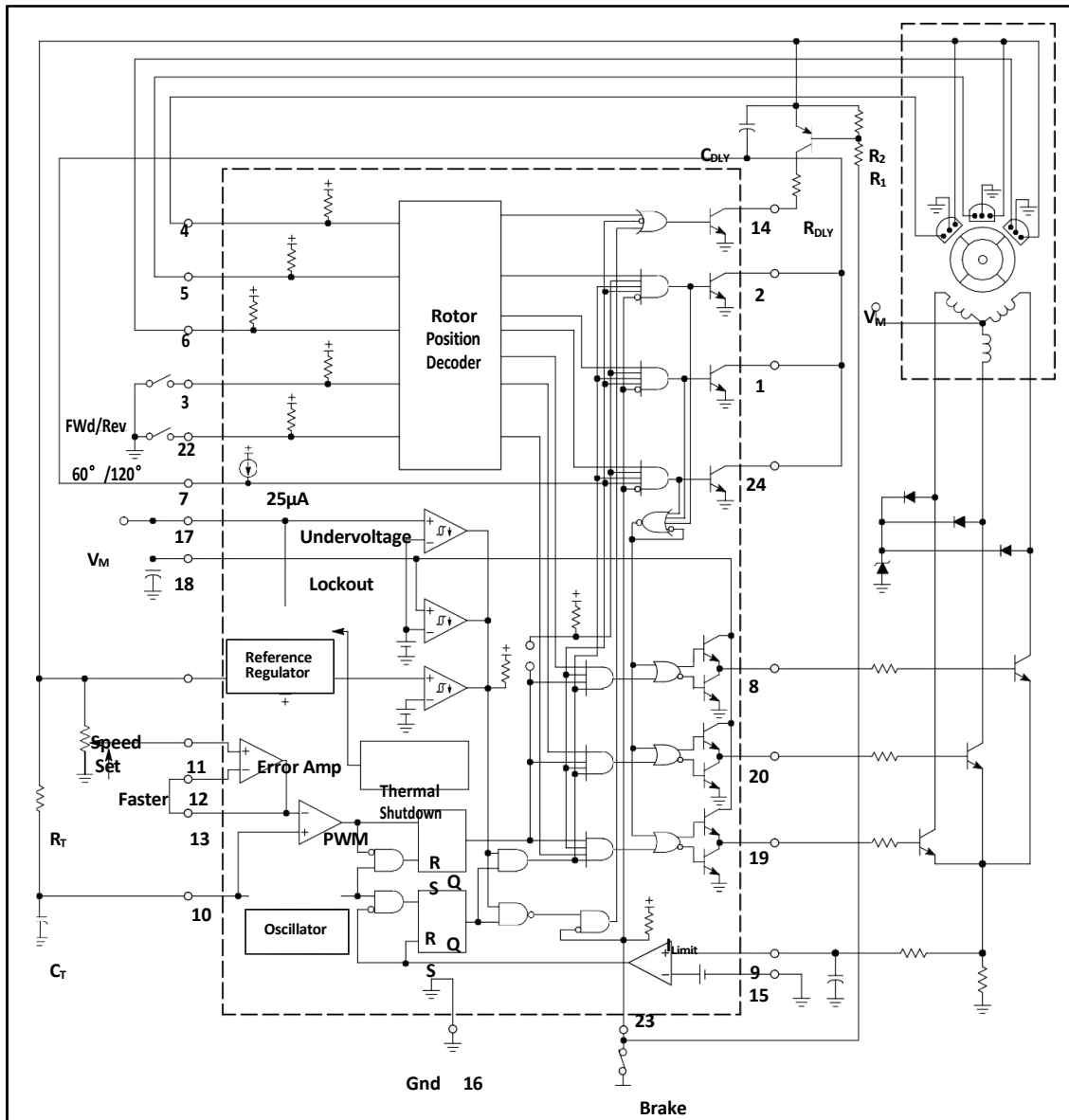
Figure 40. Three Phase, Three Step, Half Wave Motor Controller
