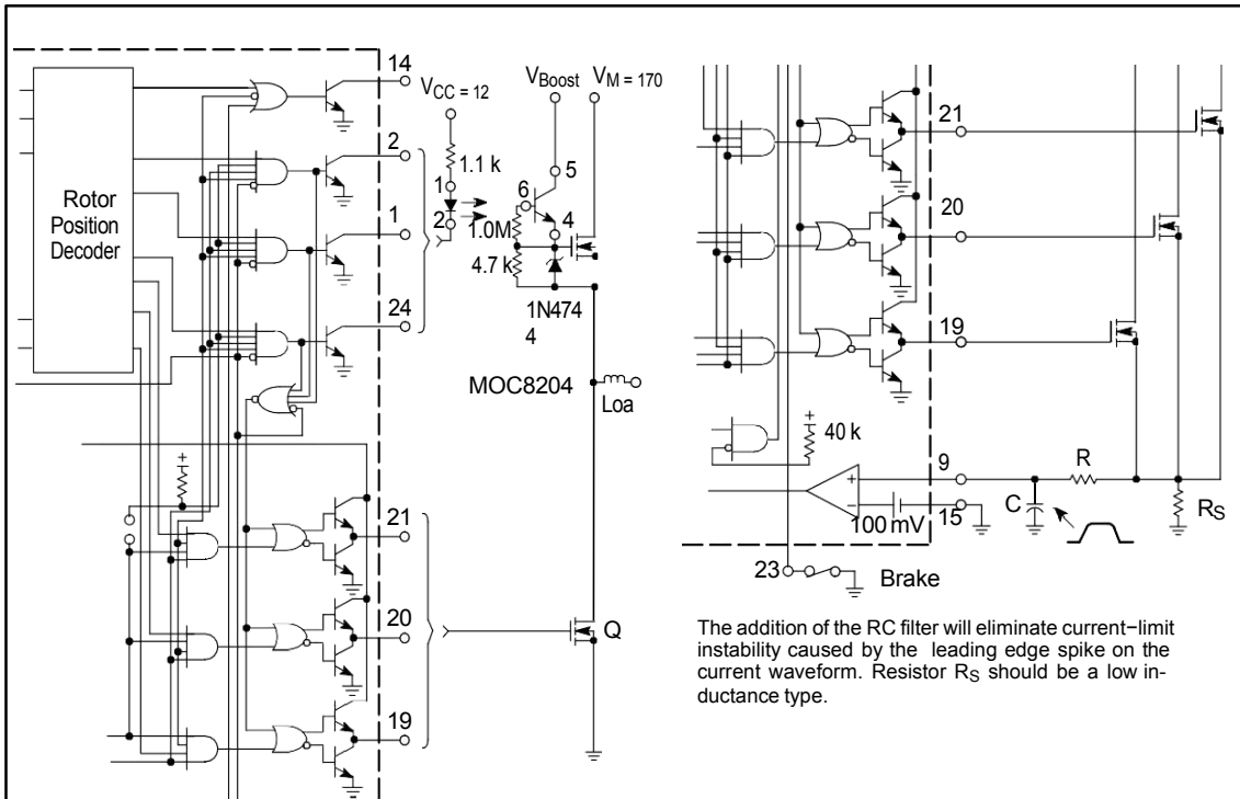
Figure 28. Current Waveform Spike Suppression
