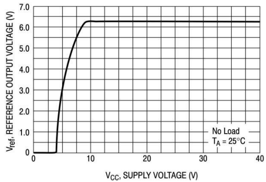
Figure 11. Reference Output Voltage versus Supply Voltage
