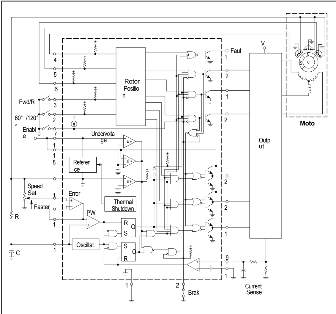
Figure 3 .Block Diagram
