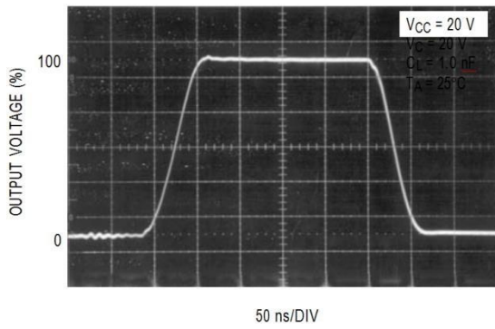
Figure 18. Bottom Drive Output Waveform
