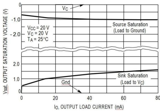
Figure 20. Bottom Drive Output Saturation Voltage versus Load Current
