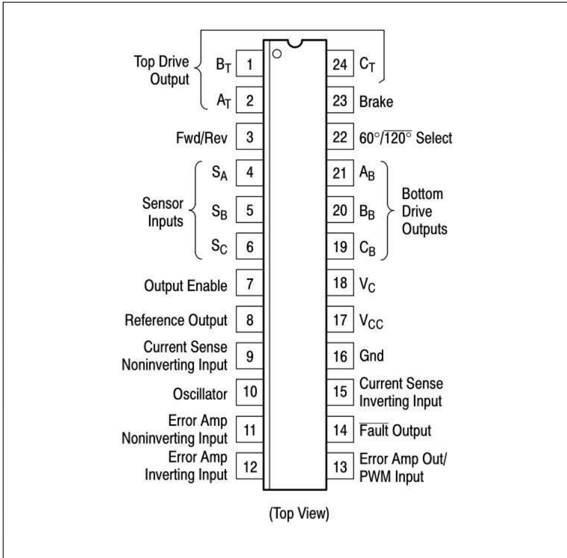
Figure 1 . PIN CONNECTIONS
