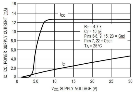
Figure 21. Power and Bottom Drive Supply Current versus Supply Voltage
