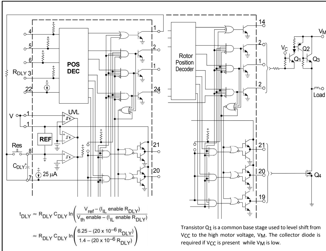
Figure 25. Timed Delayed Latched Over Current Shutdown
