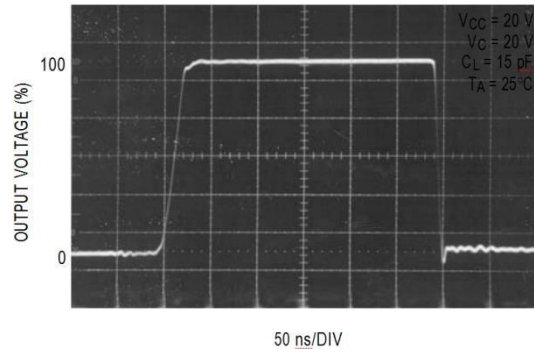
Figure 19. Bottom Drive Output Waveform
