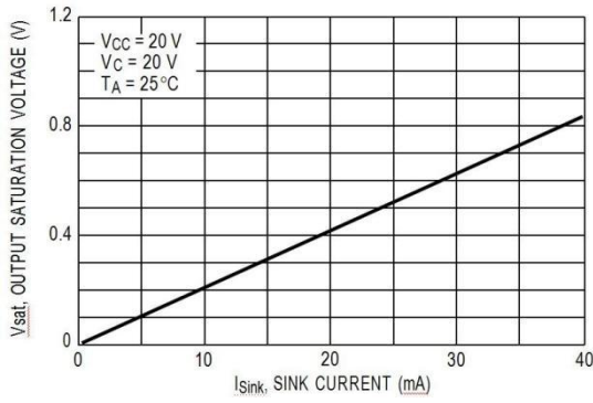
Figure 16. Top Drive Output Saturation Voltage versus Sink Current
