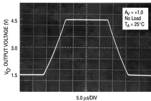
Figure 9. Error Amp Large-Signal Transient Response
