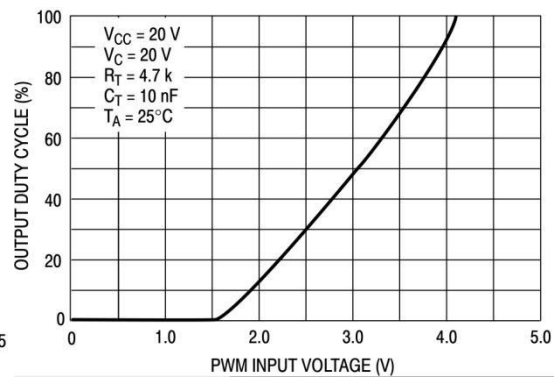
Figure 13. Output Duty Cycle versus PWM Input Voltage
