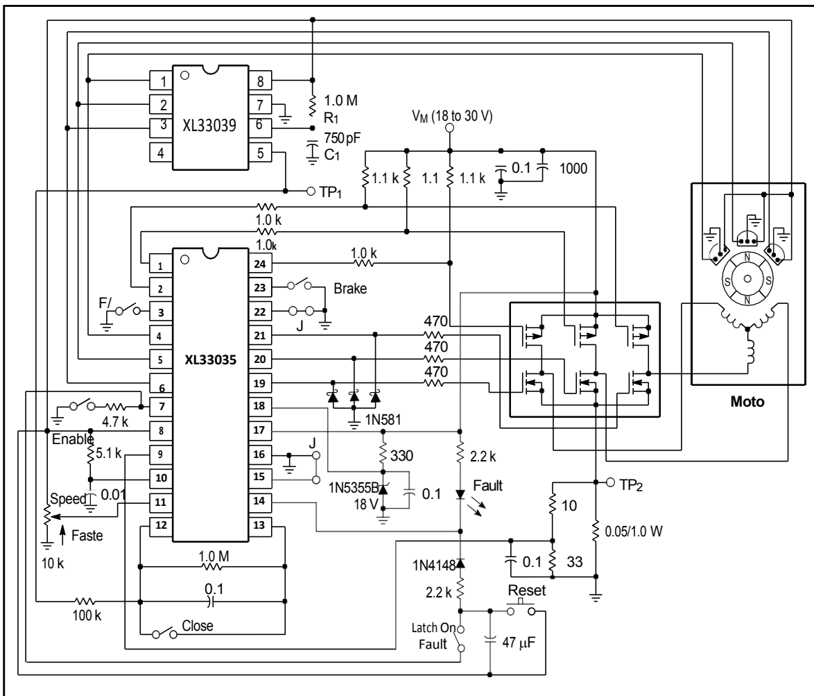
Figure 41. Closed Loop Brushless DC Motor Control Using The XL33035 and XL33039
