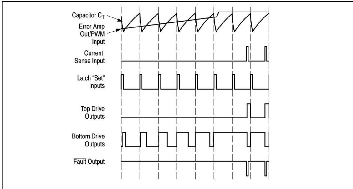
Figure 23. Pulse Width Modulator Timing Diagram Reference
