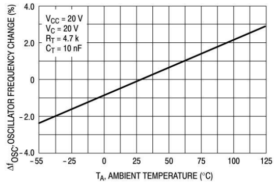
Figure 5. Oscillator Frequency Change versus Temperature
