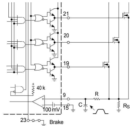
The addition of the RC filter will eliminate current-limit instability caused by the leading edge spike on the current waveform. Resistor R_S should be a low inductance type.
