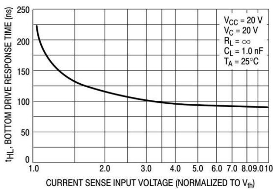
Figure 14. Bottom Drive Response Time versus Current Sense Input Voltage
