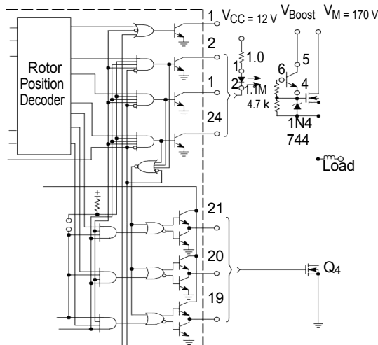
Series gate resistor R_g will dampen any high frequency oscillations caused by the MOSFET input capacitance and any series wiring induction in the gate-source circuit. Diode D is required if the negative current into the Bottom Drive Outputs exceeds 50 mA.
