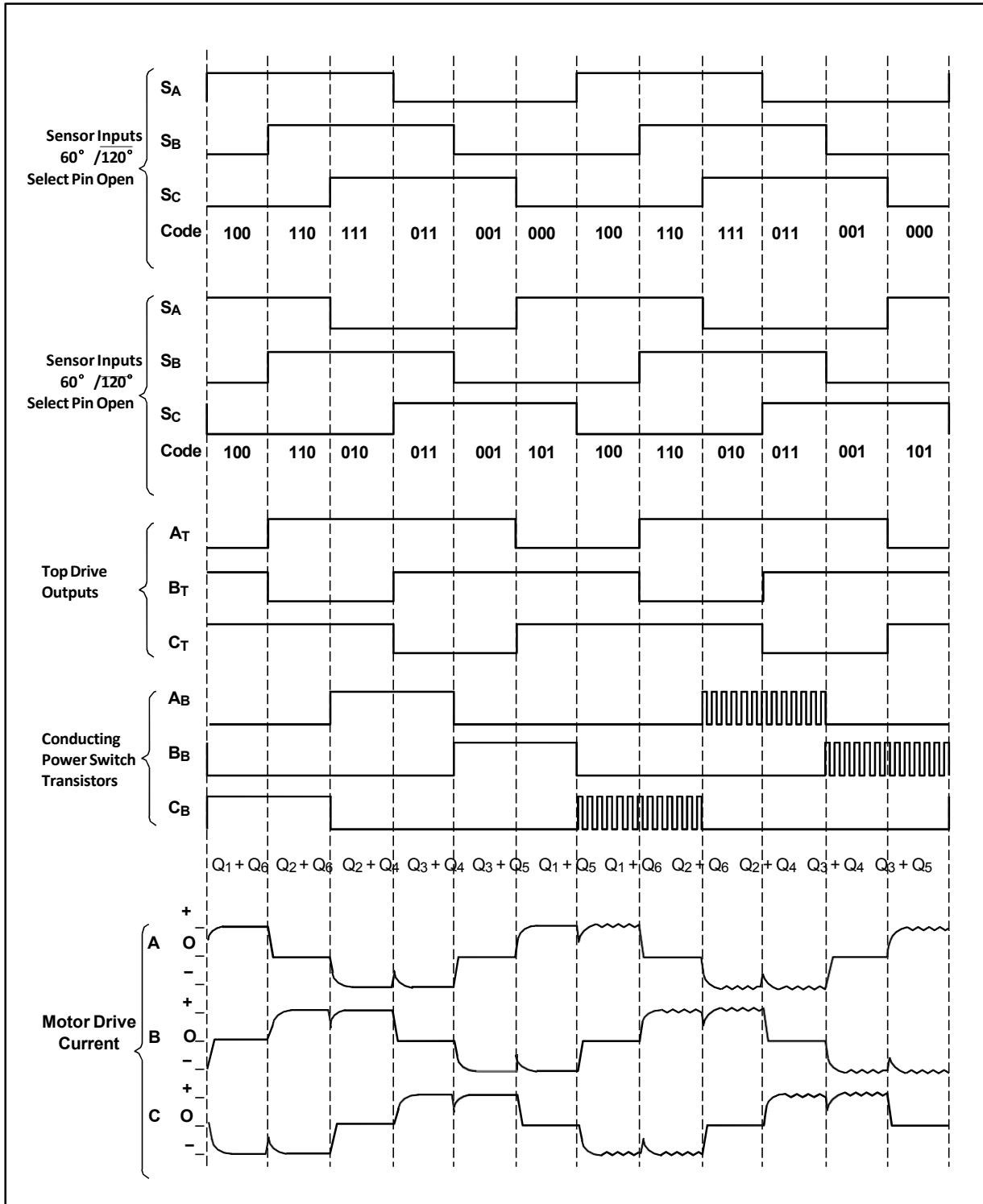
Figure 39. Three Phase, Six Step, Full Wave Commutation Waveforms
