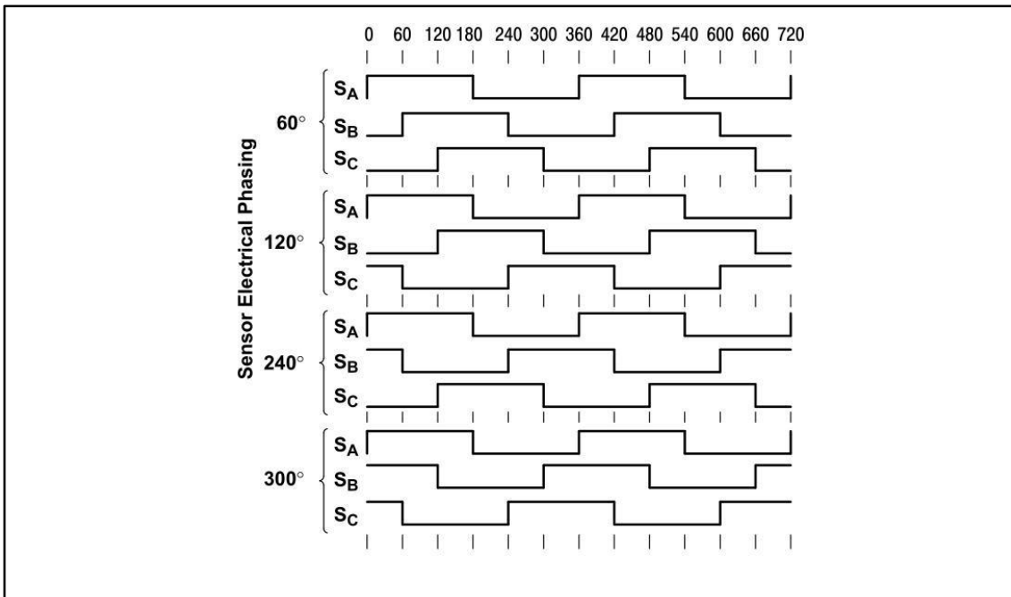
Figure 42. Sensor Phasing Comparison
