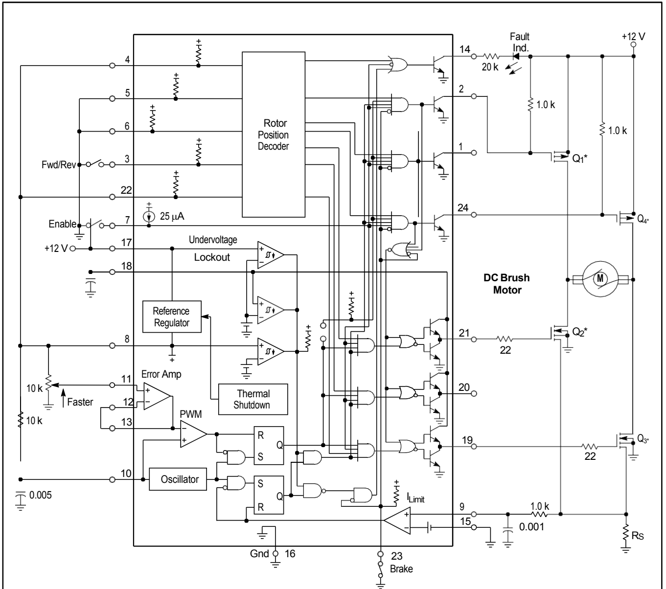
Figure 48. H-Bridge Brush-Type Controller
