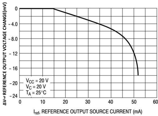
Figure 10 : Reference Output Voltage Change versus Output Source Current
