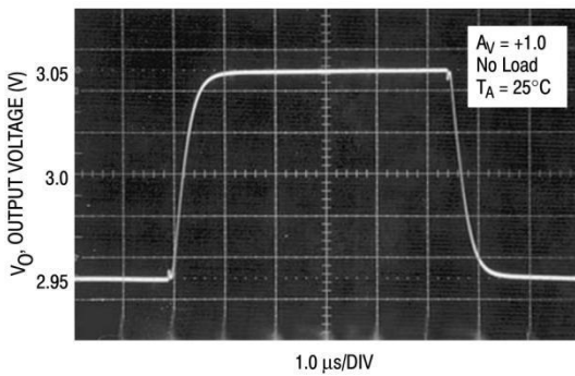
Figure 8. Error Amp Small-Signal Transient Response
