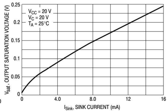
Figure 15. Fault Output Saturation versus Sink Current
