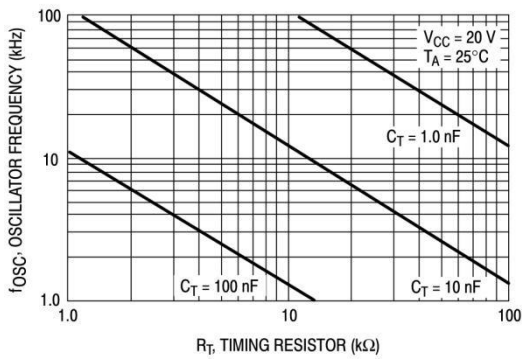
Figure 4 : Oscillator Frequency versus Timing Resistor
