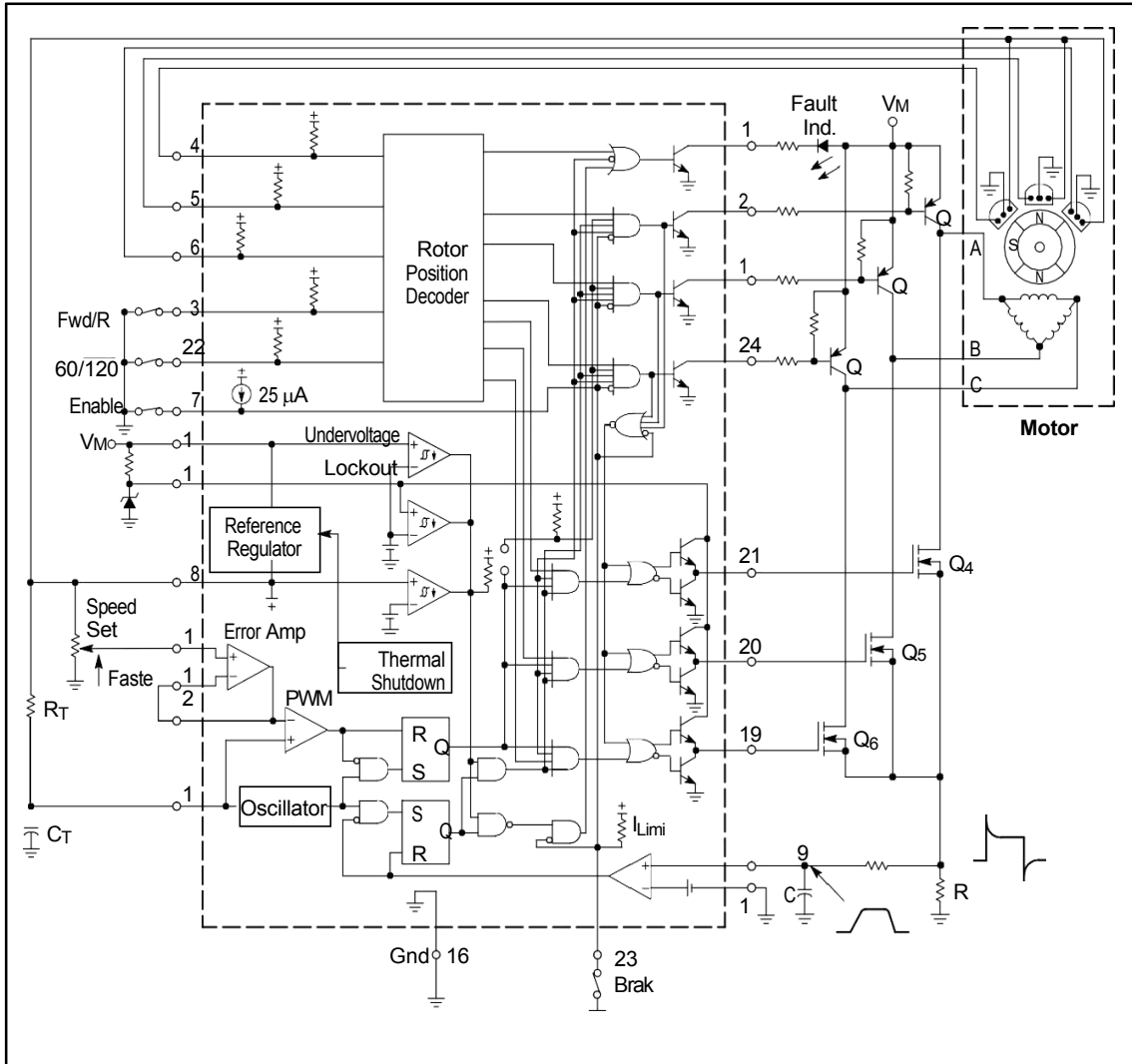
Figure 38. Three Phase, Six Step, Full Wave Motor Controller
