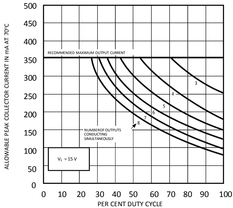
Allowable peak collector current as a function of duty cycle
