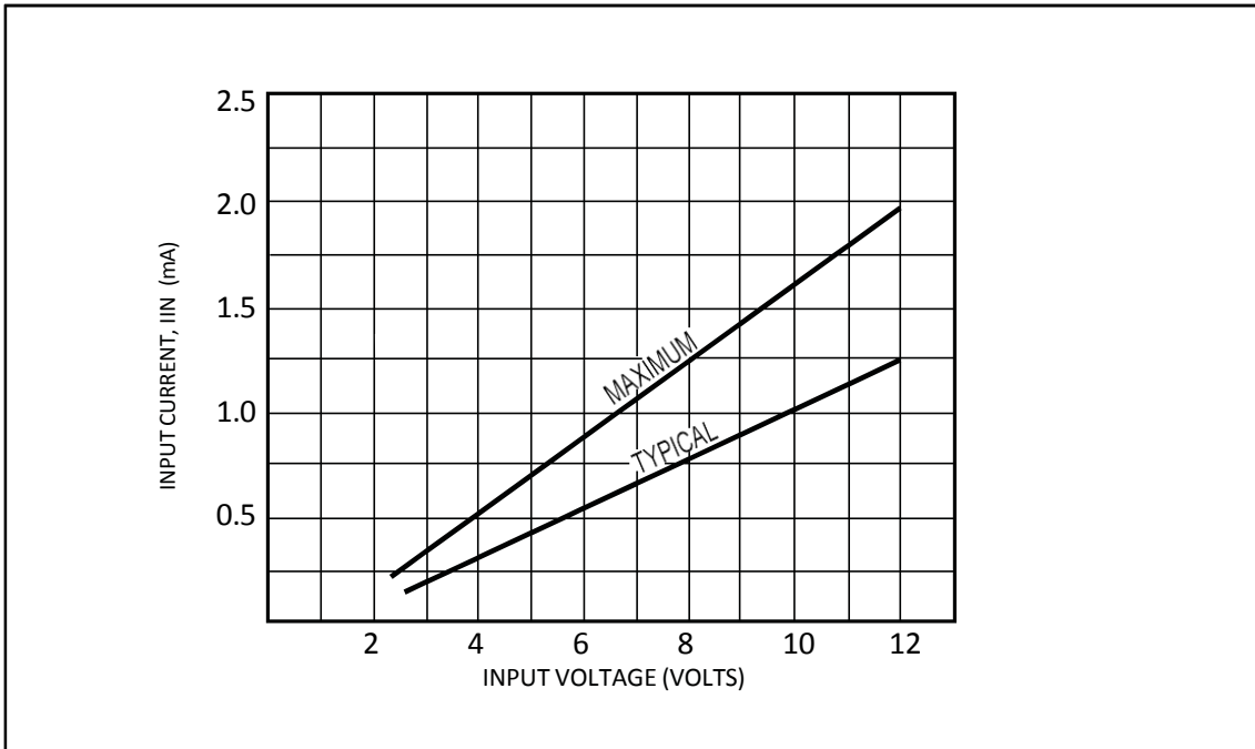
Input current as a function of input voltage
