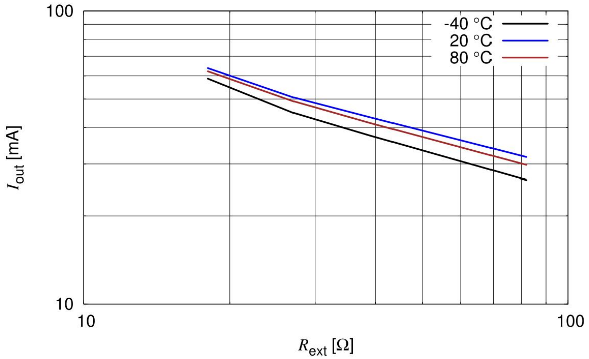
Figure 6-8 Output Current versus R_{ext} I_{out} = f(R_{ext}) , V_S = 10\text{ V} , V_S - V_{out} = 1.4\text{ V} , T_A = \text{Parameter}
