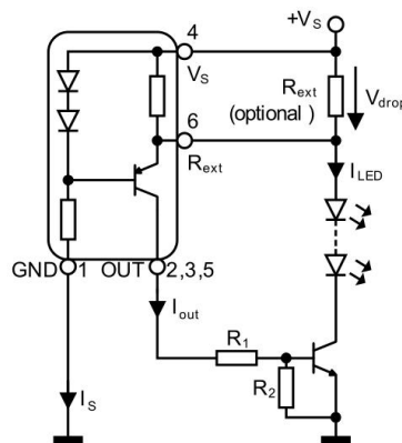
Figure 7-2 Application Circuit: Boost mode current source with external power transistor
