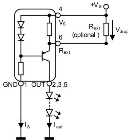
Figure 7-1 Application Circuit: Stand alone current source
