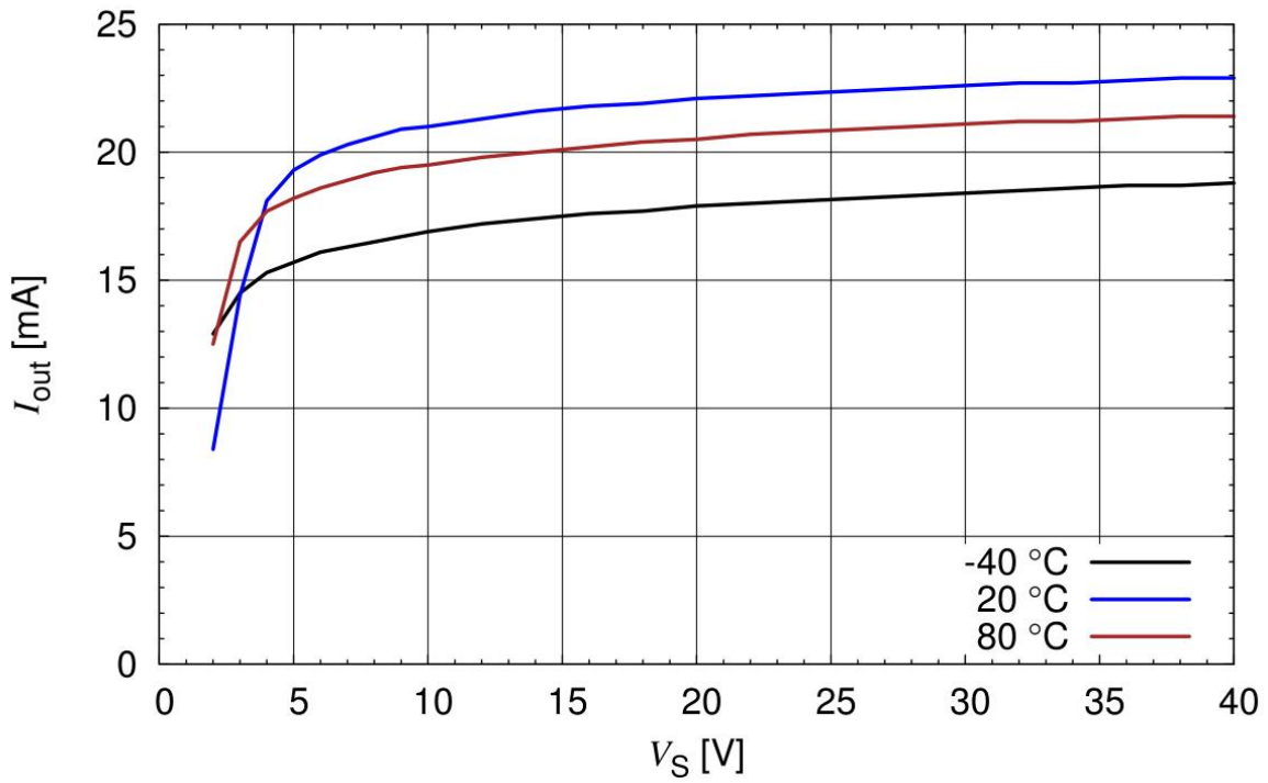
Figure 6-7 Output Current versus V_S , I_{out} = f(V_S) , V_S - V_{out} = 1.4 \text{ V} , T_A = \text{Parameter}
