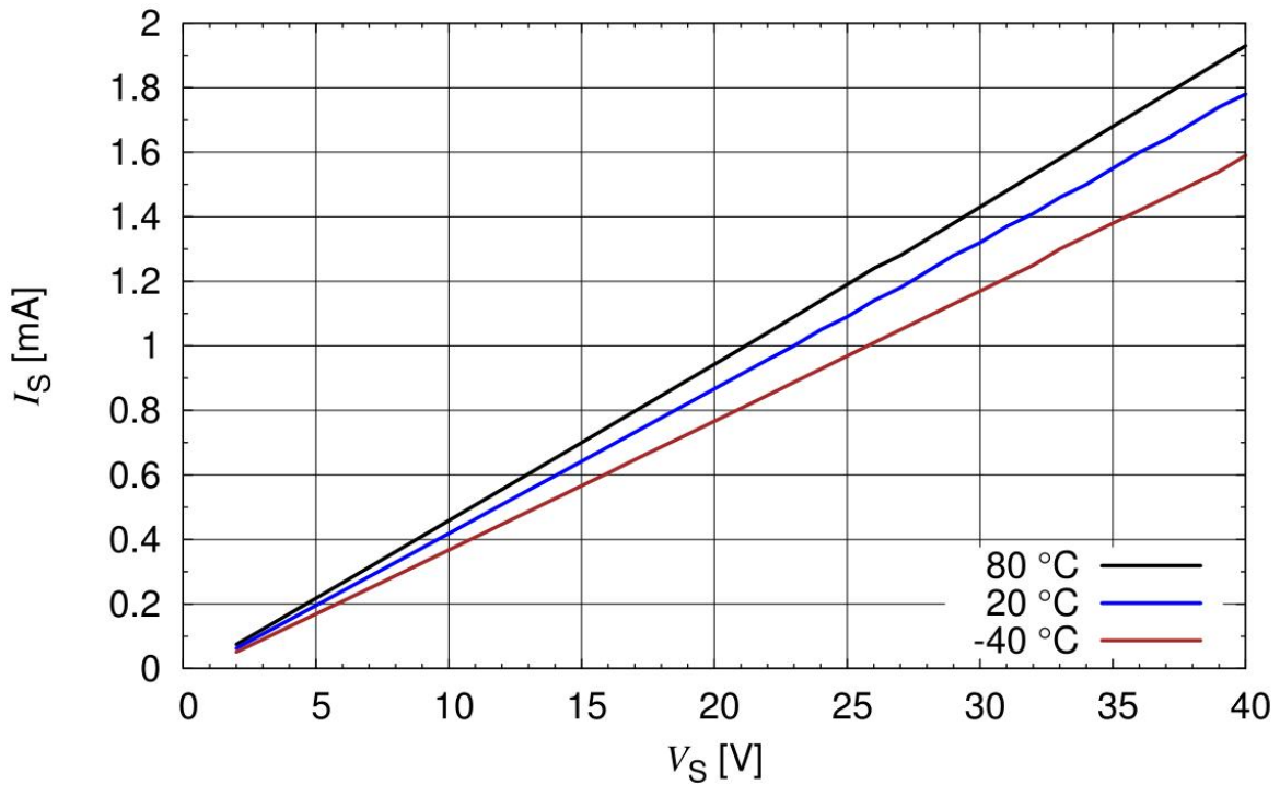
Figure 6-5 Supply Current versus V_S , I_S = f(V_S) , T_A = \text{Parameter}
