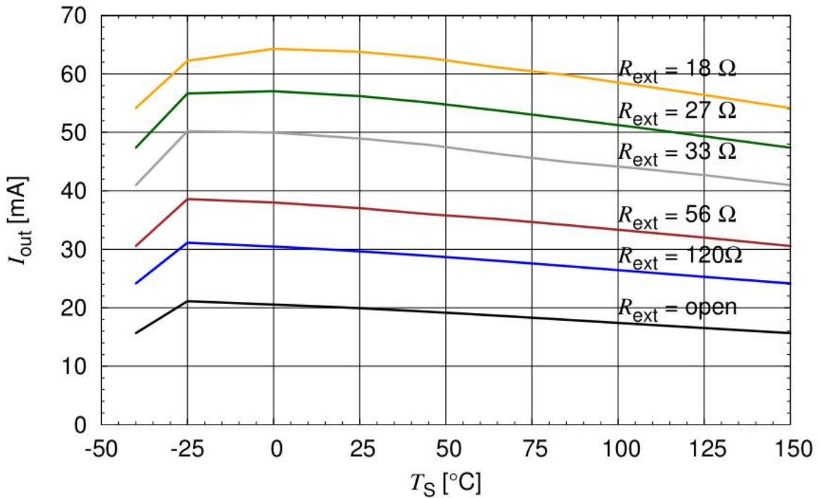
Figure 6-9 Output Current versus T_S I_{out} = f(T_S) , V_S = 10\text{ V} , V_S - V_{out} = 1.4\text{ V} , R_{ext} = \text{Parameter}
