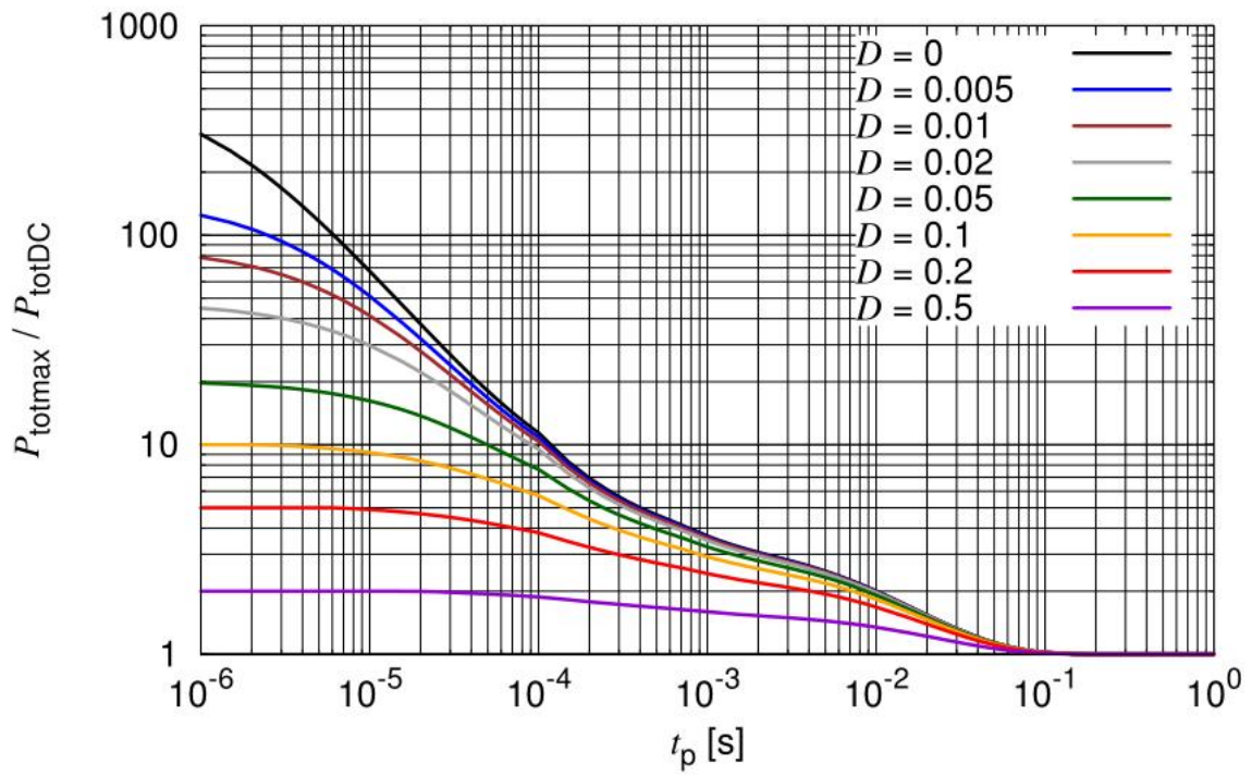
Figure 6-3 Permissible Pulse Load P_{\text{totmax}} / P_{\text{totDC}} = f(t_p)
