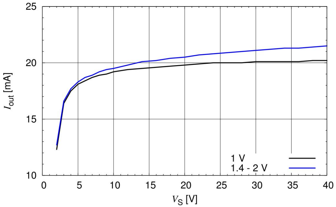
Figure 6-6 Output Current versus V_S , I_{out} = f(V_S) , V_S - V_{out} = \text{Parameter}
