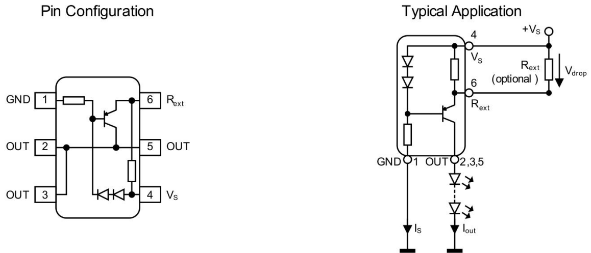
Figure 4-1 Pin configuration and typical application
