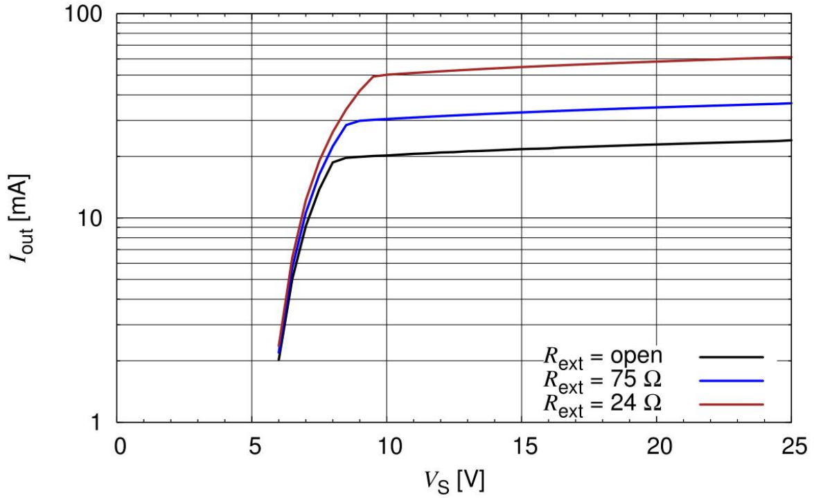
Figure 6-4 Output Current versus V_S , I_{out} = f(V_S) , V_S - V_{out} = 1.4 \text{ V} , R_{ext} = \text{Parameter}
