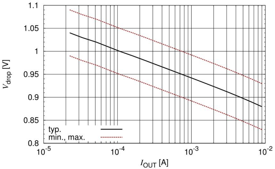
Figure 6-10 Reference Voltage V_{drop} vs I_{out} V_{drop} = f(I_{out}) , I_{out} = 10 \mu\text{A} to 10 \text{ mA}
