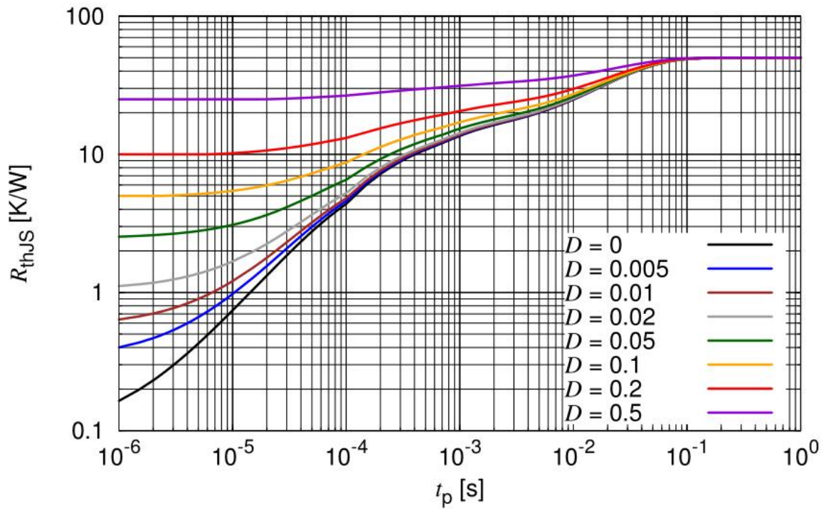
Figure 6-2 Permissible Pulse Load R_{thJS} = f(t_p)
