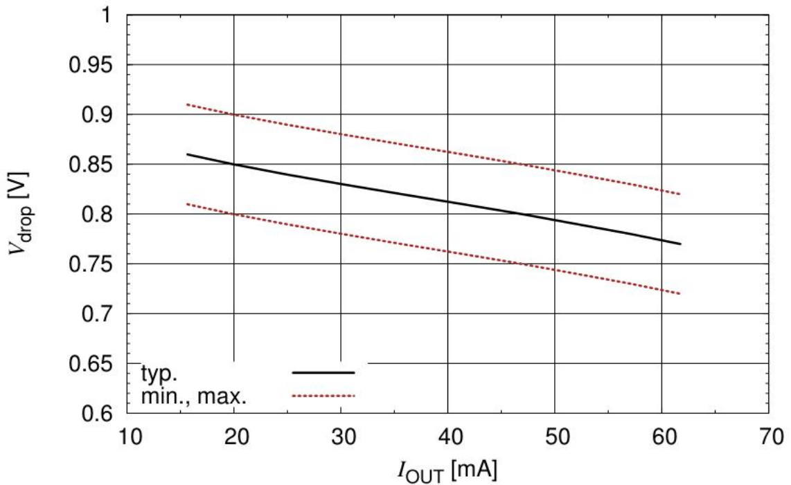
Figure 6-11 Reference Voltage V_{drop} vs I_{out} V_{drop} = f(I_{out}) , I_{out} = 10 \text{ mA} to 65 \text{ mA}
