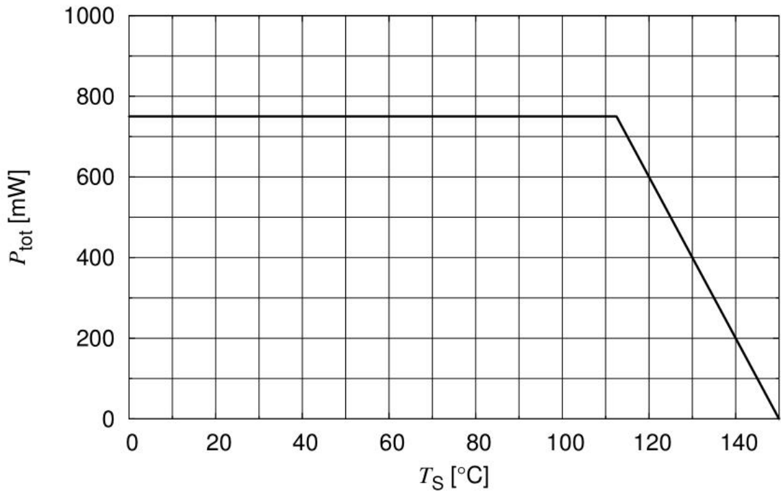
Figure 6-1 Total Power Dissipation P_{tot} = f(T_S)
