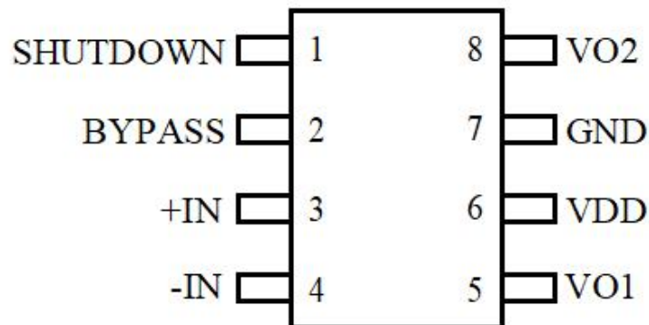
SOP-8/MSOP-8
