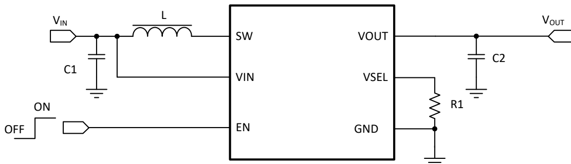
Typical Application
