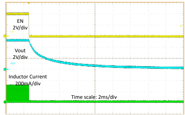
V_{IN} = 3.6V V_{OUT} = 5V R_{load} = 500\Omega Figure 8-7. Shutdown by EN
