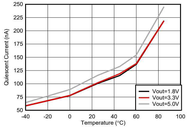
Figure 6-8. Quiescent Current into VOUT vs Temperature
