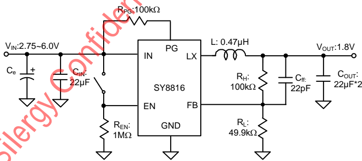
Figure 1. Schematic Diagram
