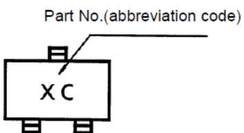
Fig. 9.3 Marking RN1303
