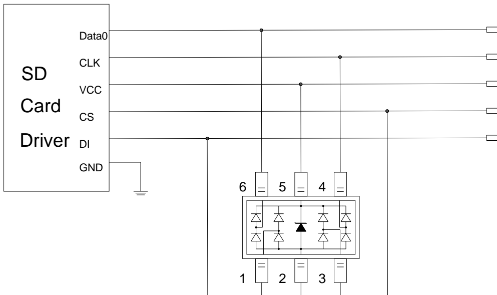
SRV05-4MR6T1G-MS Typical Interface Application
