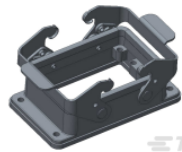
TE Part #T1419320000-000 H32A-AG
