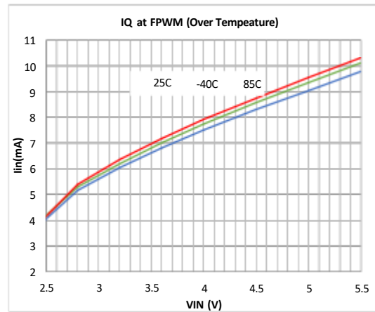
图18. I_q vs V_{IN} 过热, Mode=High, V_{OUT} = 1.8V
