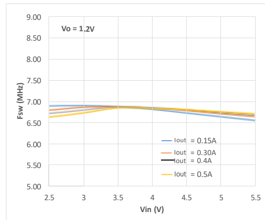
图22. FSW, V_{OUT} = 1.2V , Mode=High
