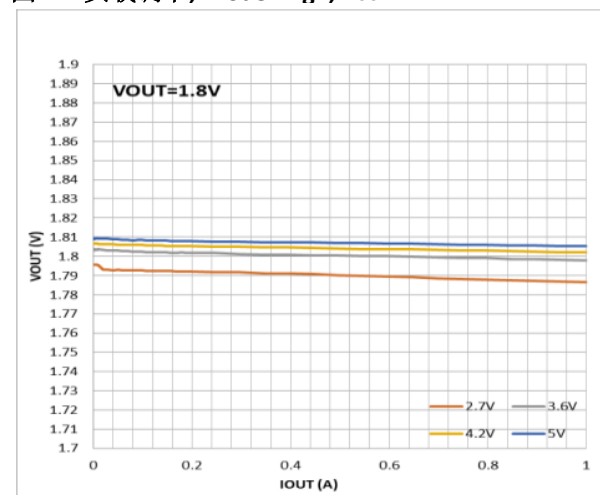
图14. 负载调节, Mode=High, V_{OUT} = 1.8V
