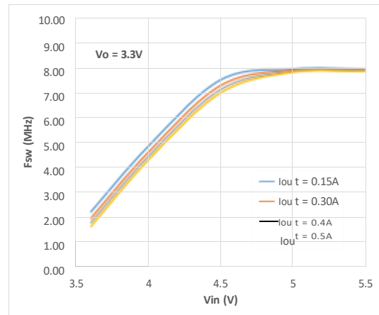
图26. FSW, V_{OUT} = 3.3V , Mode=High
