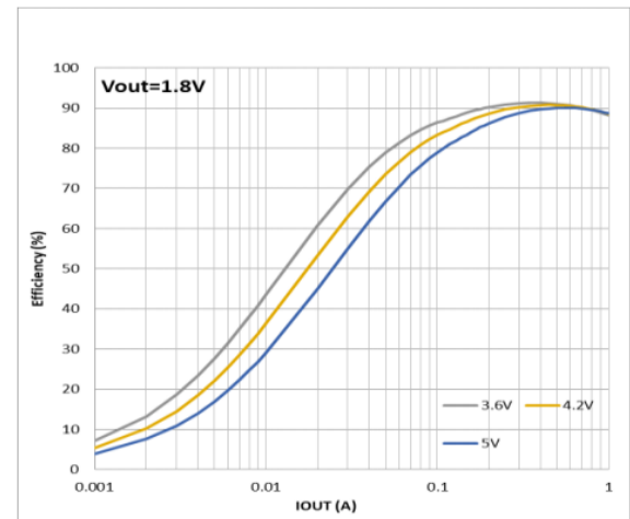
图8. Efficiency, Mode=High, V_{OUT} = 1.8V
