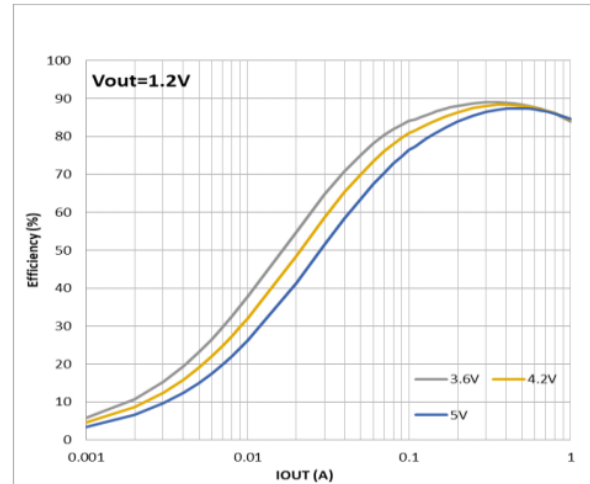
图 6. Efficiency, Mode=High, V_{OUT} = 1.2V
