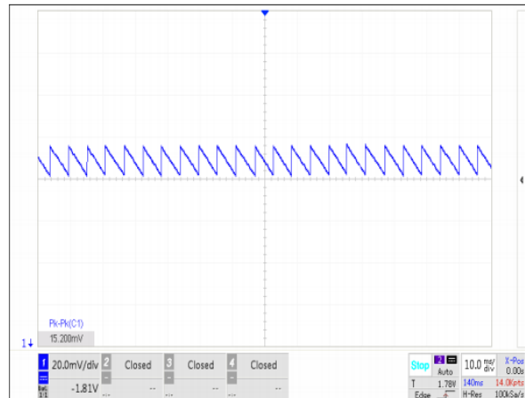
图30. 输出电压纹波, V_{OUT} = 1.8V , Mode=Low, I_{LOAD}=0A
