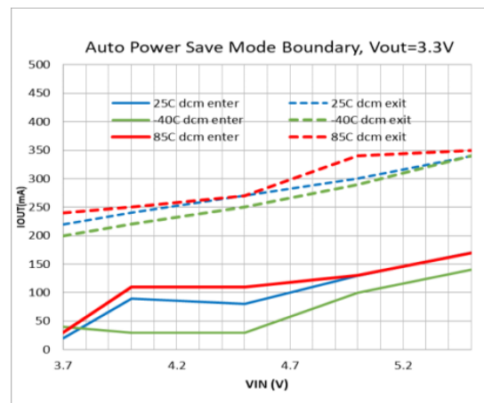
图20. PFM/PWM Boundaries, Mode=Low, V_{OUT} = 3.3V
