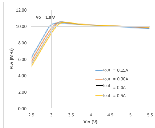
图24. Fsw, V_{OUT} = 1.8V , Mode=High
