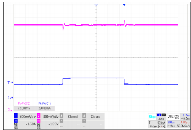
图34. 负载瞬变, V_{OUT} = 1.8V , Mode=Low, I_{LOAD} = 500mA to 750mA
