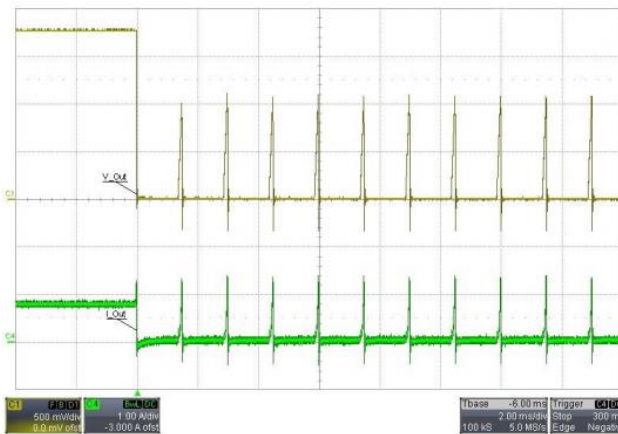
图37. OCP hiccup: V_{IN} = 3.6V , V_{OUT} = 1.8V
