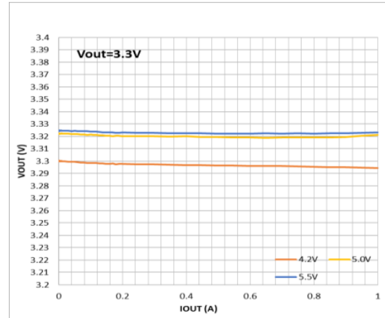
图16. 负载调节, Mode=High, V_{OUT} = 3.3V
