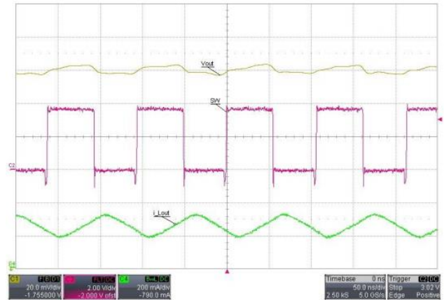
图40. PWM Mode Operation: V_{IN} = 3.6V , V_{OUT} = 1.8V , I_{LOAD} = 300mA
