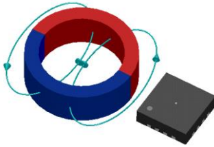
Figure 5: Side-Shaft Mounting
