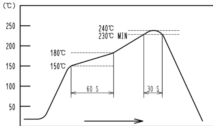
⚠ Fig - 2 Recommended reflow profile temperature (temperature at SMT leads)
