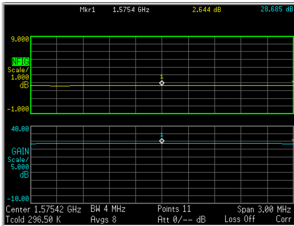
Figure 10. LNA Noise figure @3.0V
