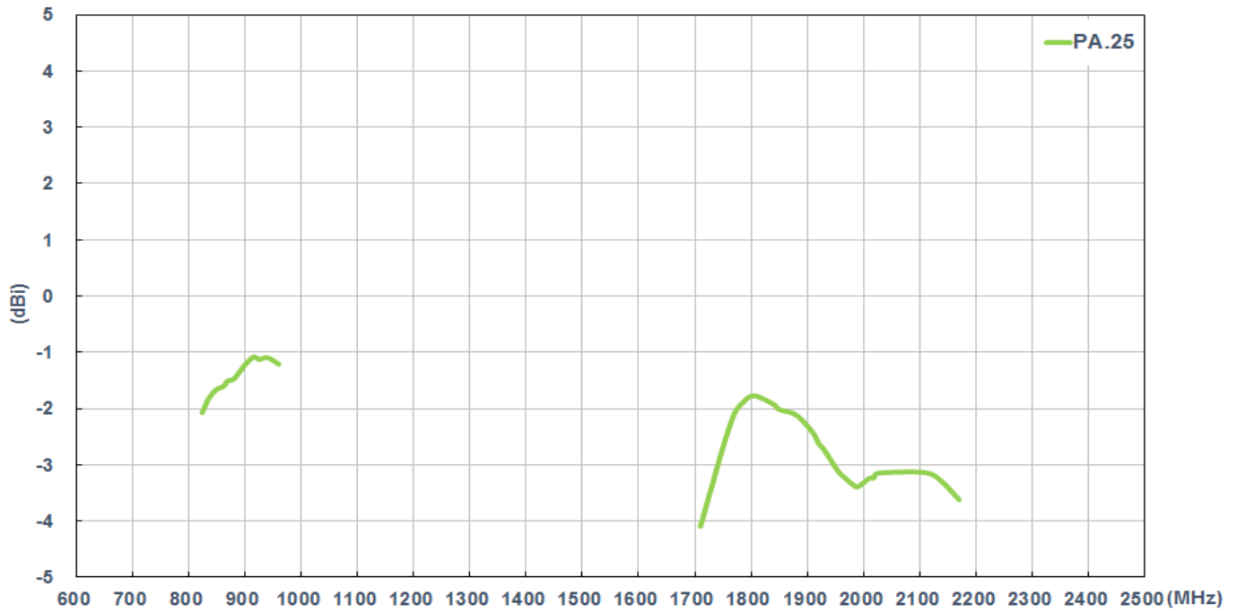
Figure 6. Average Gain of the PA.25 Cellular Antenna
