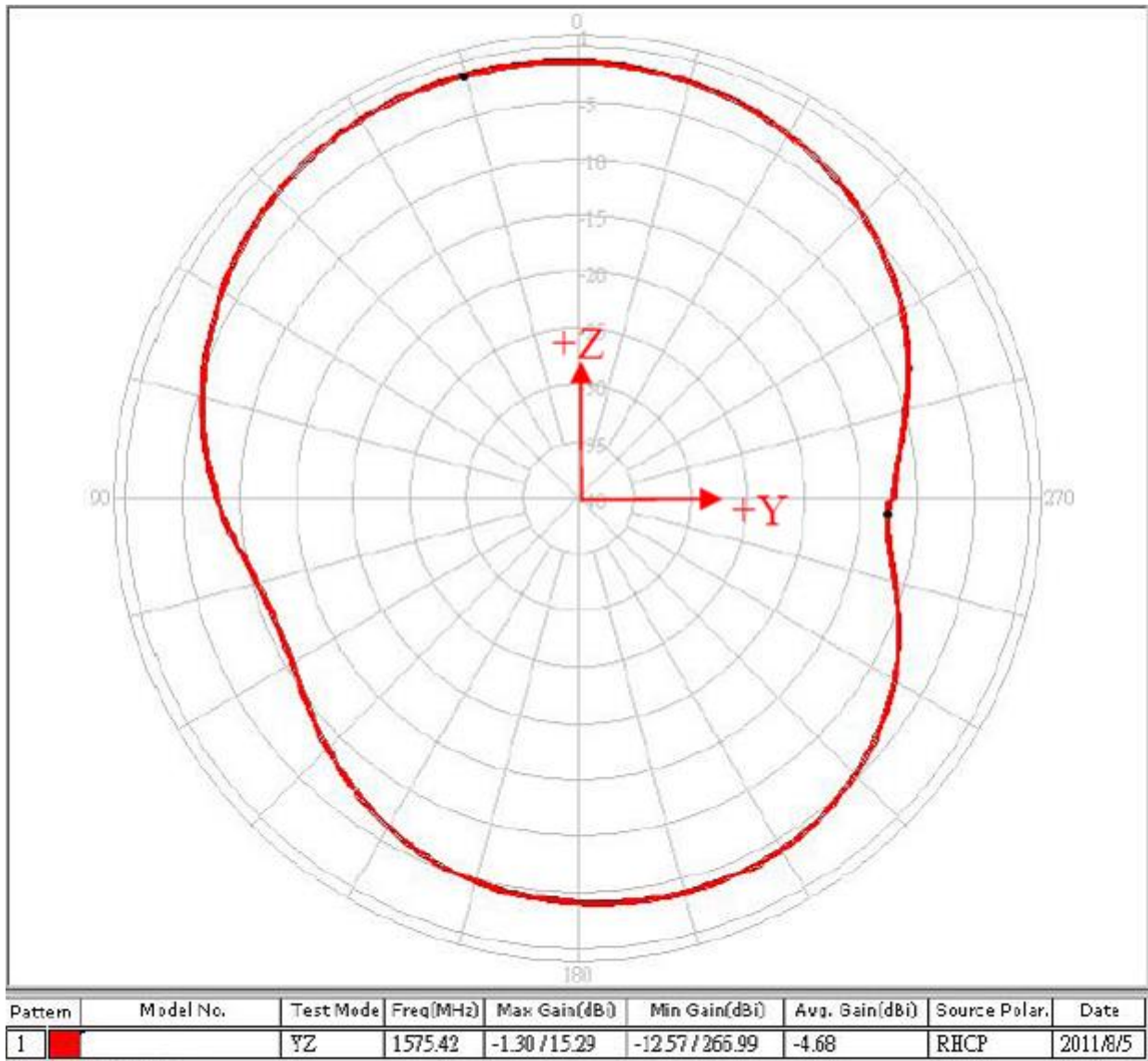
Figure 12. Y-Z plane
