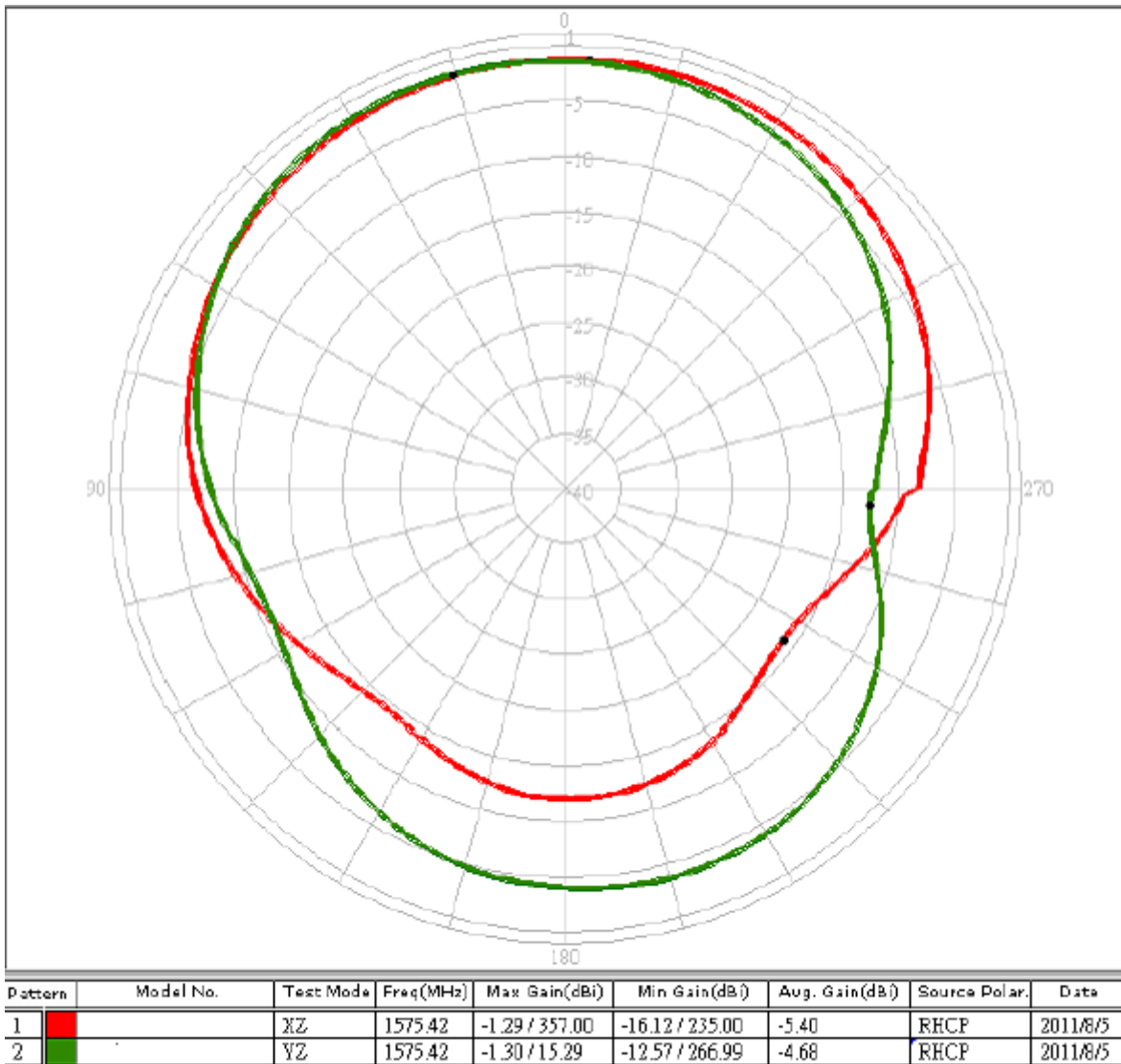
Figure 13. X-Y plane
