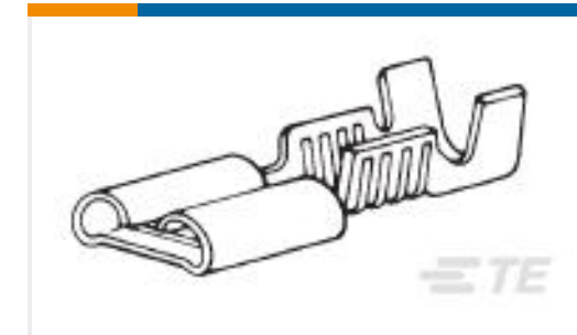
TE Part #60904-2 205 FASTON REC 22-18 AWG TPBR
