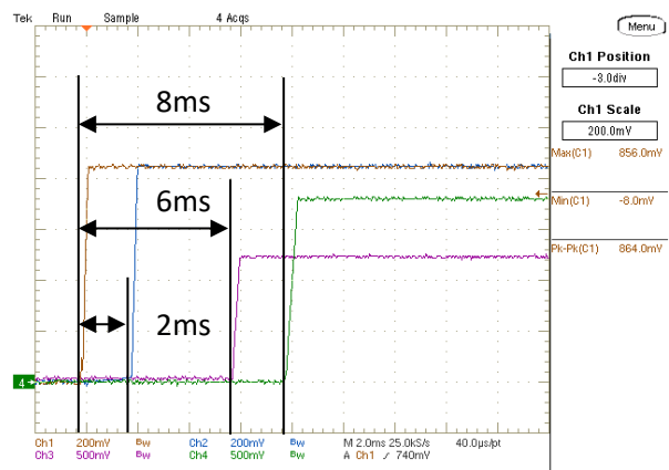
On/Off Enable Delay (Vin=5.0V, Iout=MAX) Trace1=Vout1, Trace2=Vout2, Trace3=Vout3, Trace4=Vout4
