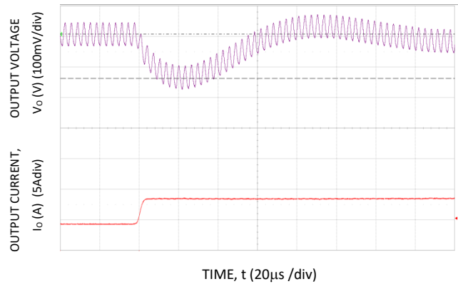
Figure 16. Transient Response to Dynamic Load Change from 50% to 100% at 28Vin, Cext – 1x22µF+1x470µF, CTune=1.5nF & RTune=200
