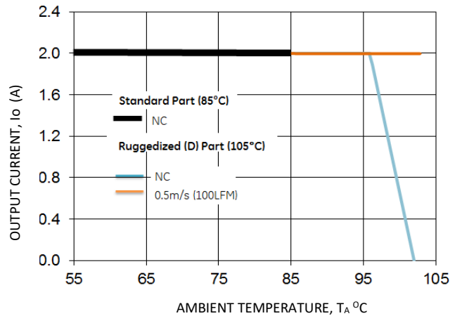
Figure 61. Derating Output Current versus Ambient Temperature and Airflow.
