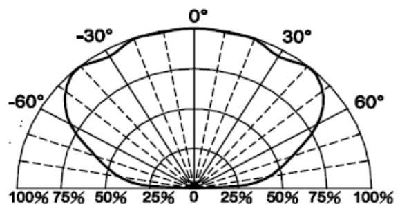
Fig.6 Directive Radiation
